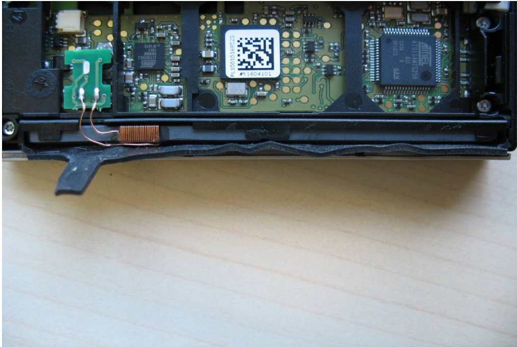
Photo 3: (coil antenna)
