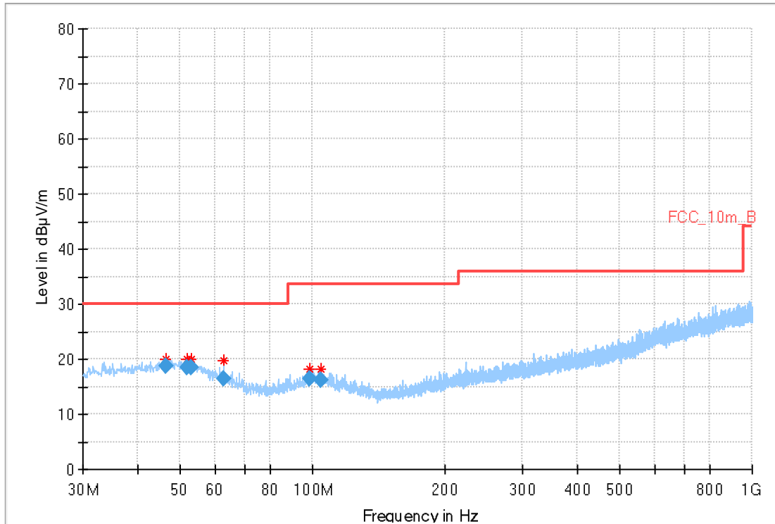
Plot 3: 30 MHz to 1 GHz, TX mode, 2480 MHz, vertical & horizontal polarization, 1 Msp
