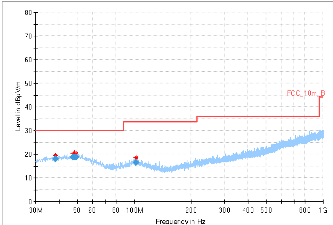
Plot 2: 30 MHz to 1 GHz, TX mode, 2440 MHz, vertical & horizontal polarization, 1 Msp
