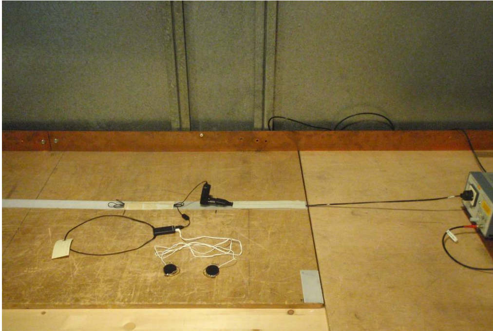
Photo 3 (Conducted emissions):
