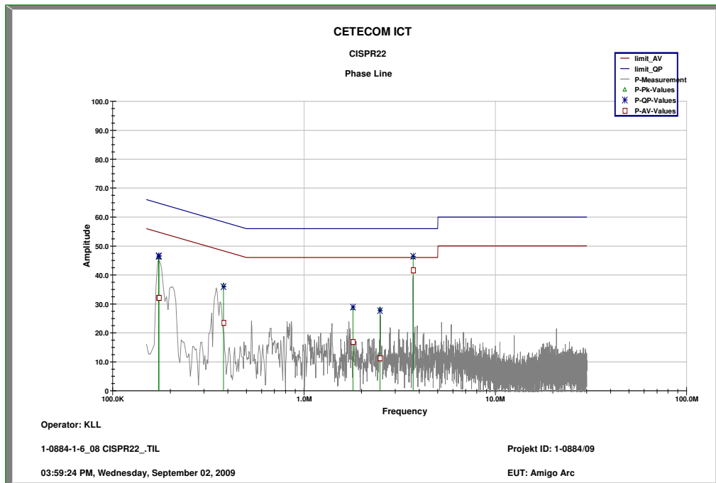
Plot 1: Charging mode, Phase Line (sample #5)
