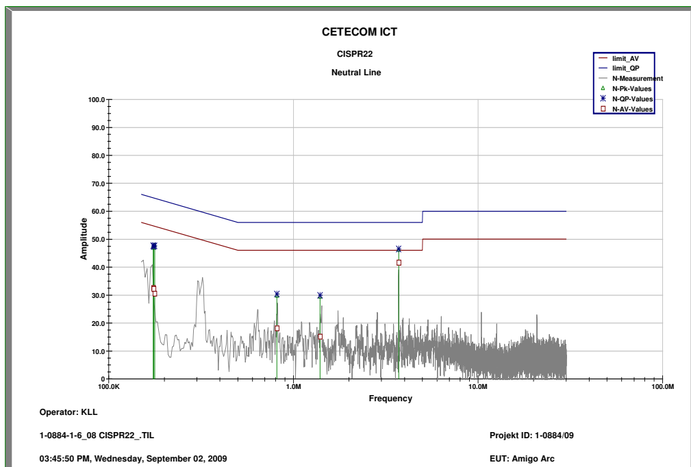
Plot 2: Charging mode, Neutral Line (sample #5)
