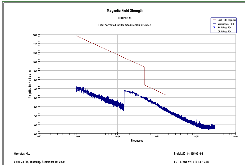
Plot 1: TX 9kHz – 30MHz
