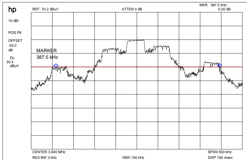
Plot 2: 20 dB-Bandwidth
