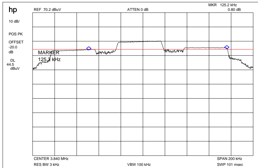
Plot 2: 20 dB-Bandwidth
