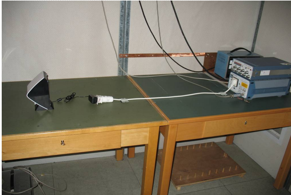
Photo 3 (Conducted Emissions):
