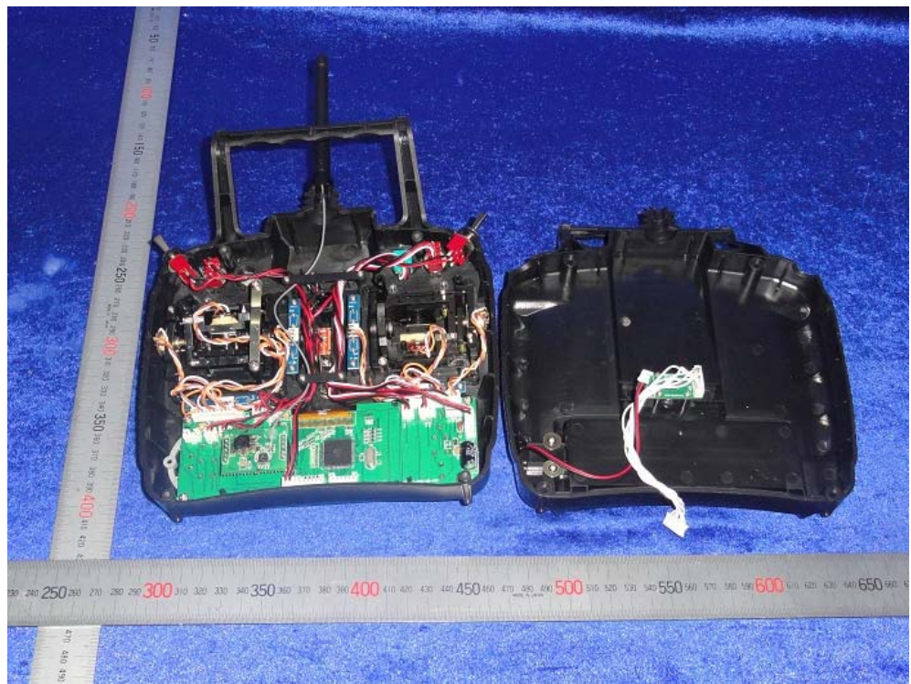
Inside view of the Tx
