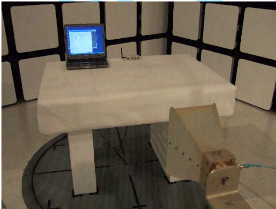
Test Configuration 1: 960 MHz to 40 GHz
