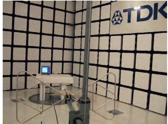
Test Configuration 2: 30 MHz to 960 MHz
