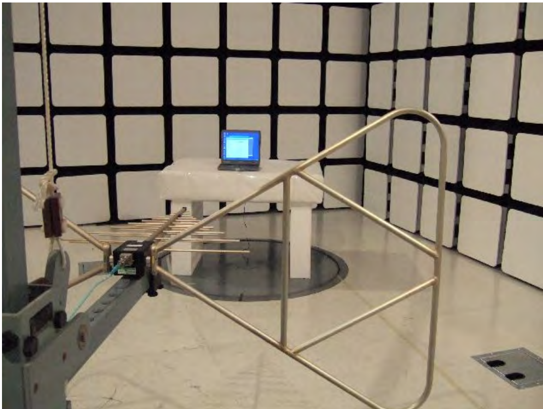
Test Configuration 2. 30 MHz to 960 MHz
