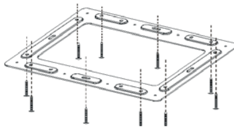
Six Screw ST4.2*16
