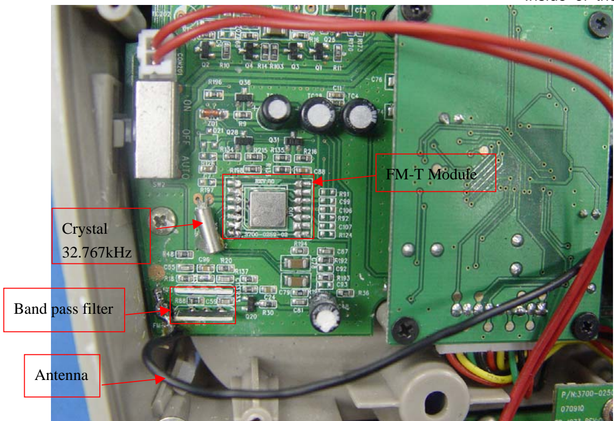
Figure 6 Inside of the EUT
