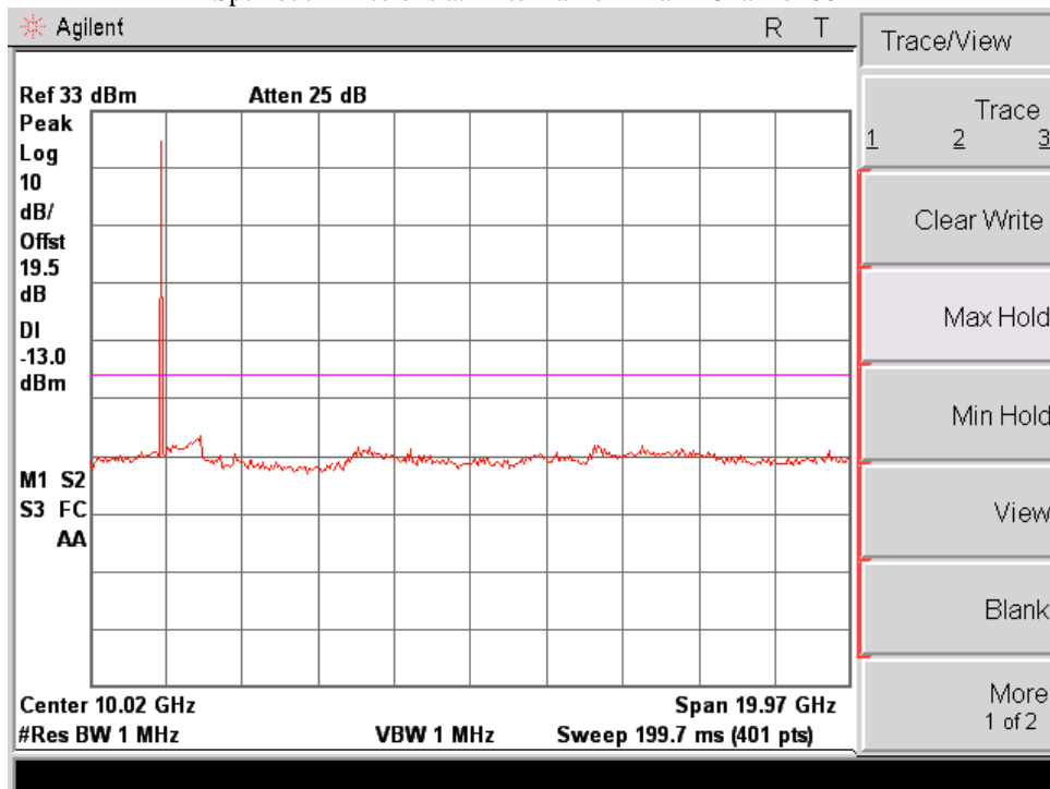
Spurious Emissions at Antenna Terminal – Channel 661
