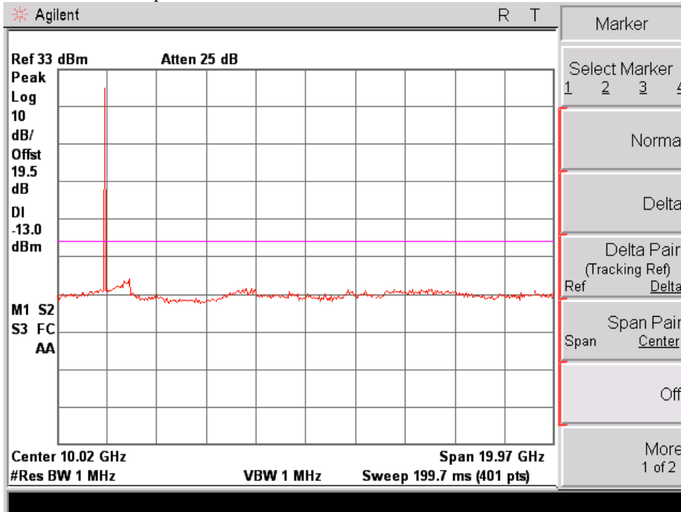
Spurious Emissions at Antenna Terminal – Channel 810
