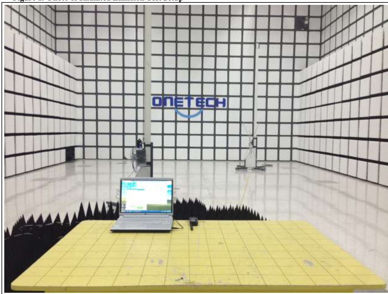
Figure 1. Photo of Radiated Emission Test Setup
