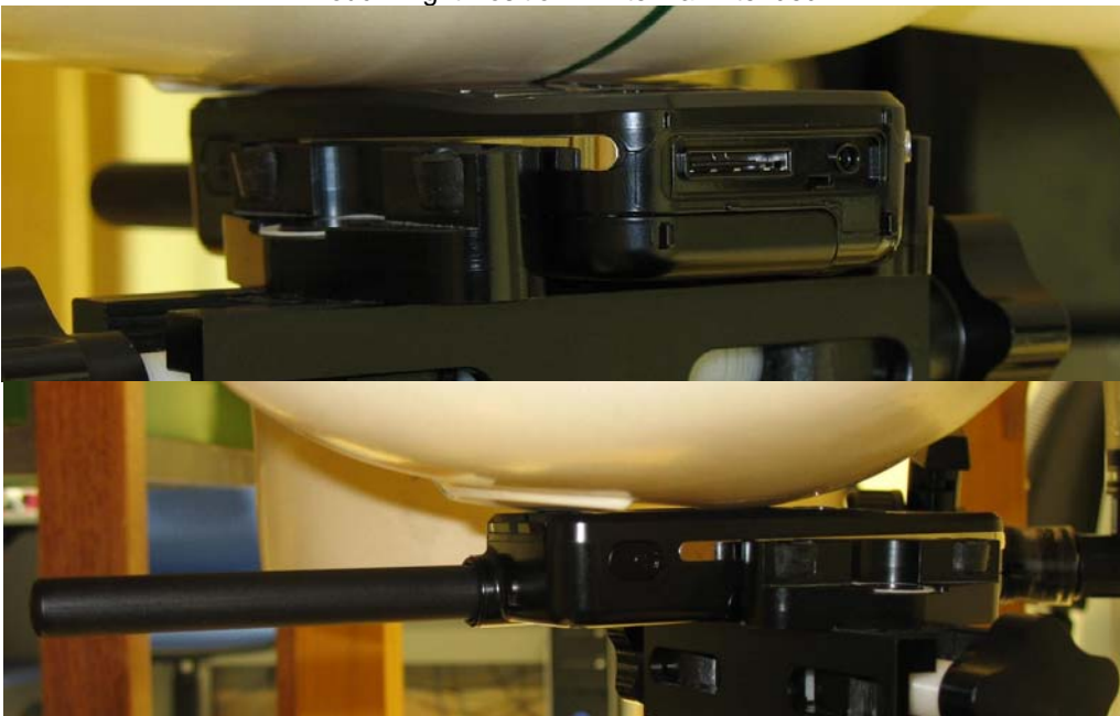
Touch Right Position - Antenna Extended
