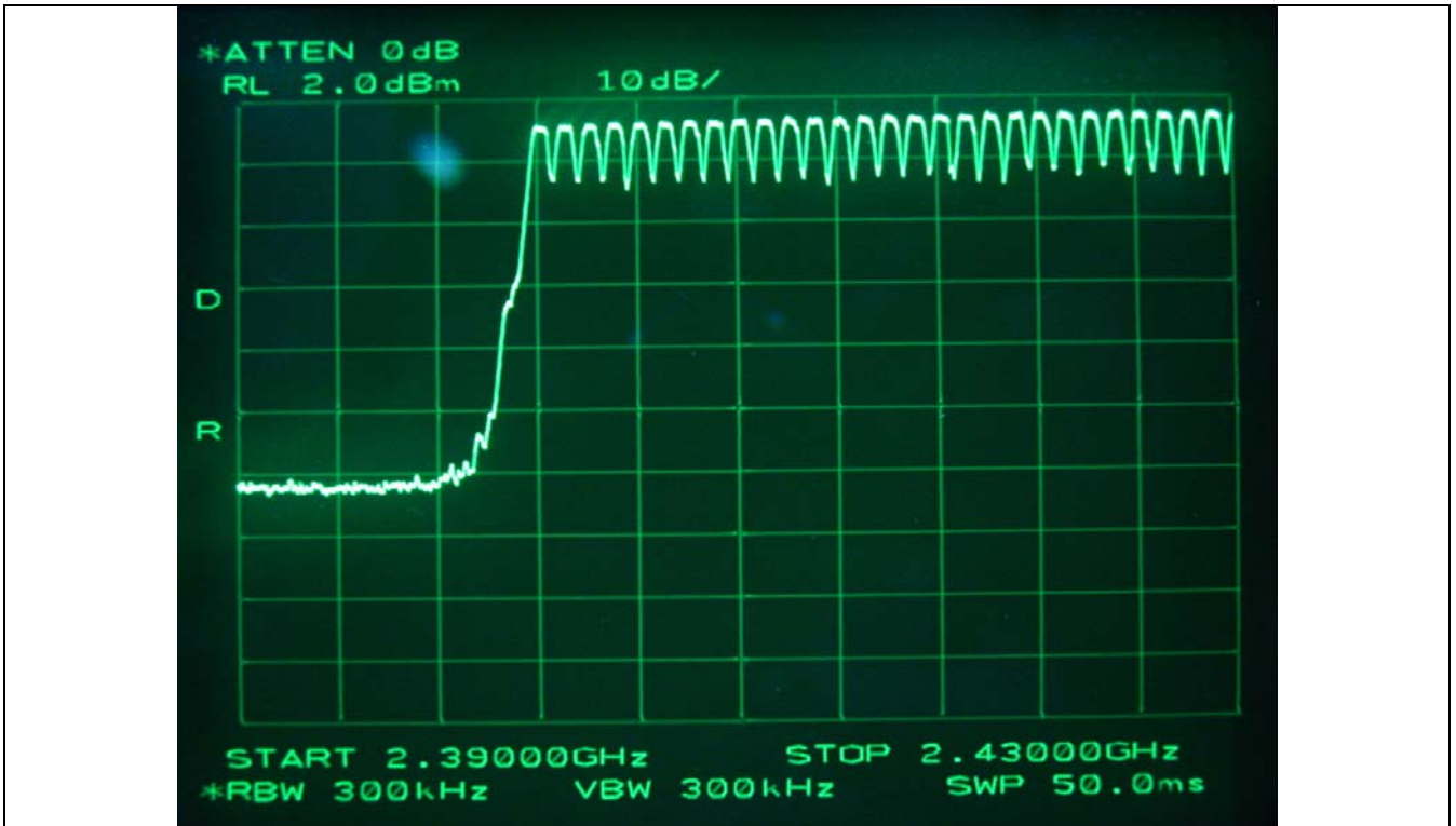
Number of hopping channel: 28
