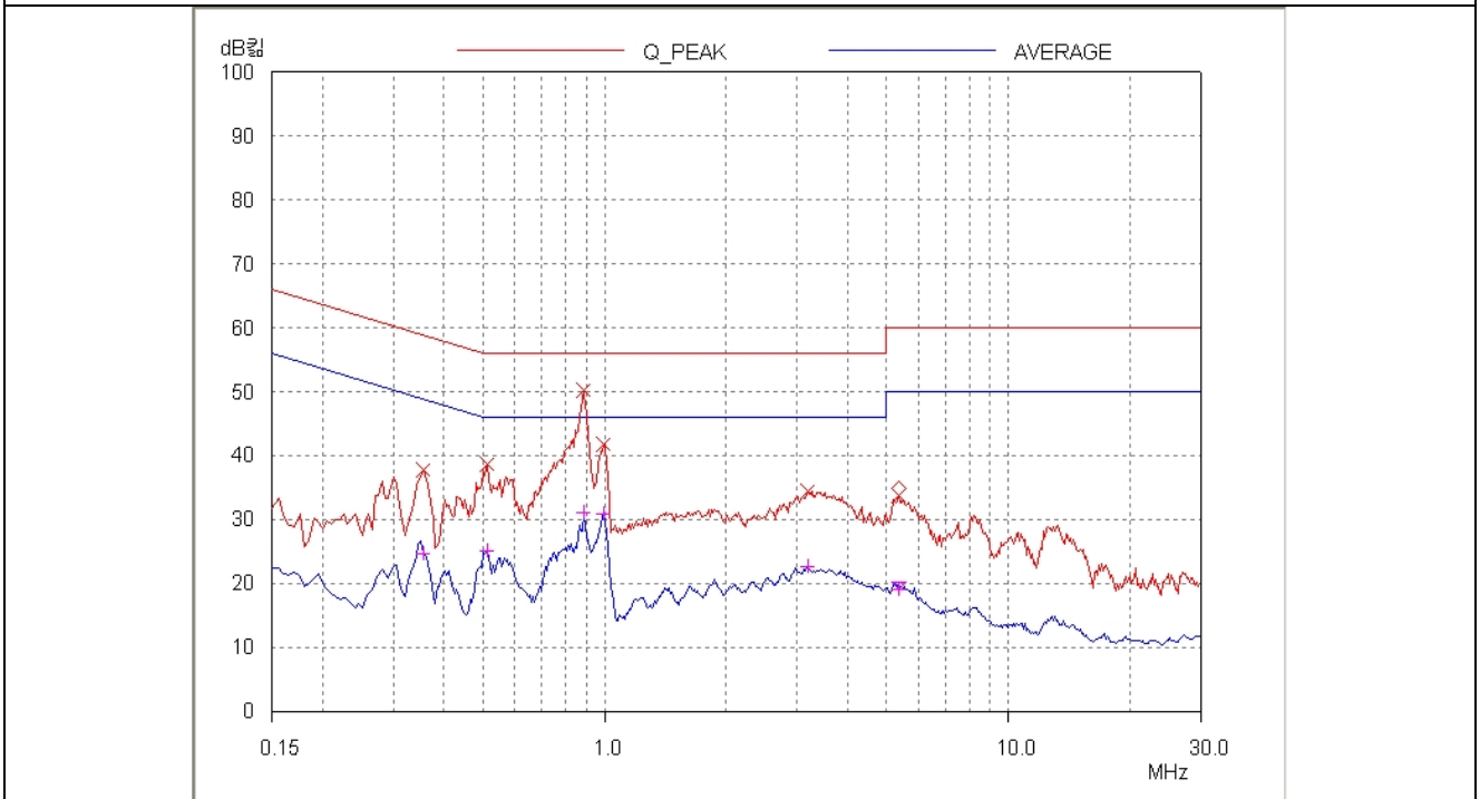
NEUTRAL LINE
