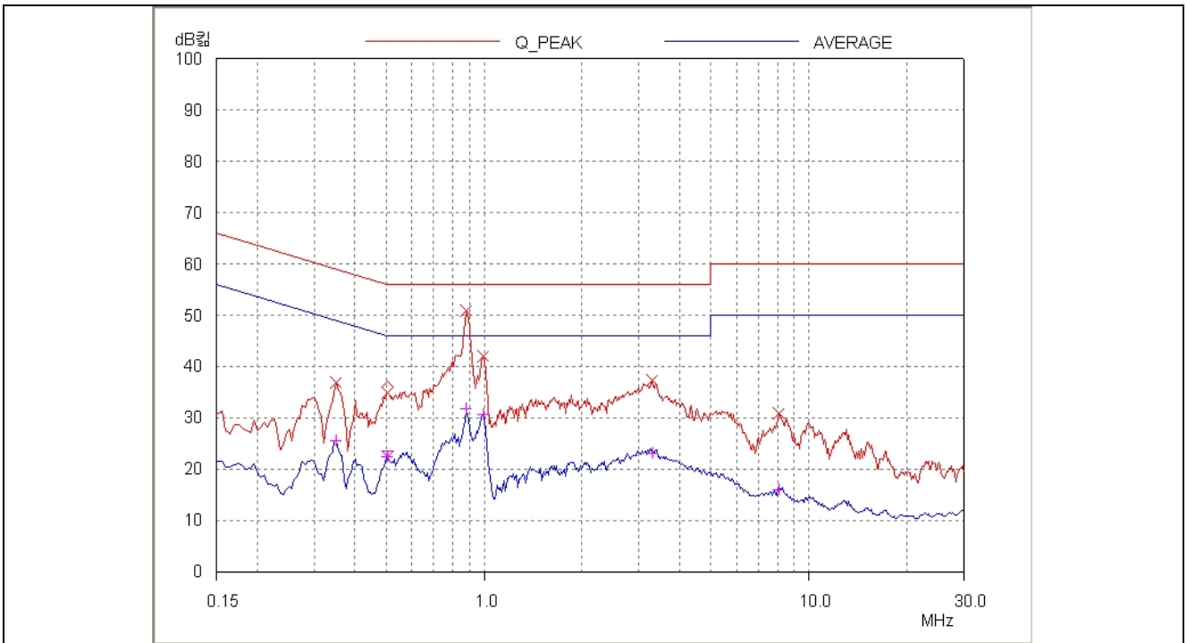
HOT LINE
