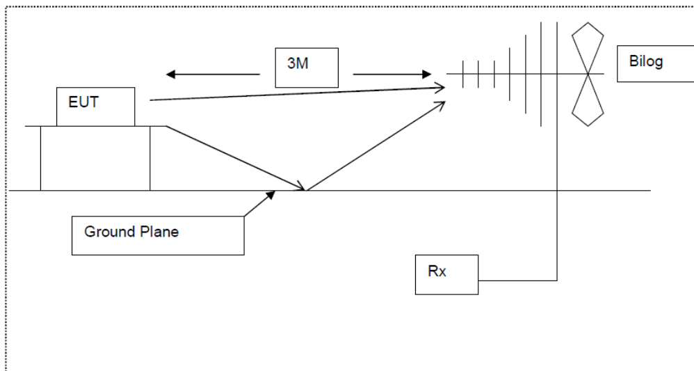
Diagram of the radiated emissions test setup.
