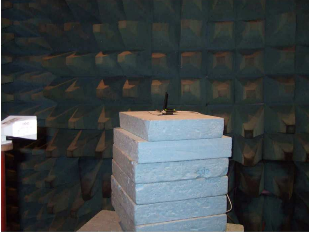
Photograph of radiated emissions set-up 18-26GHz
