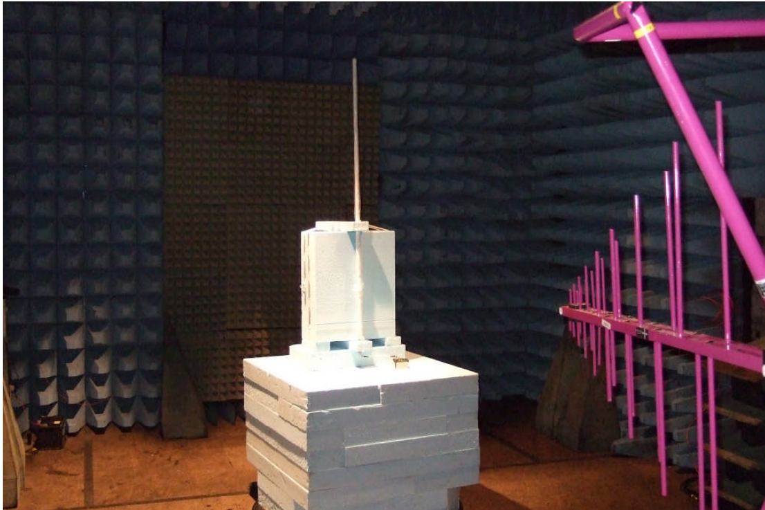
Photograph of the EUT as viewed from in front of the antenna, site M.
