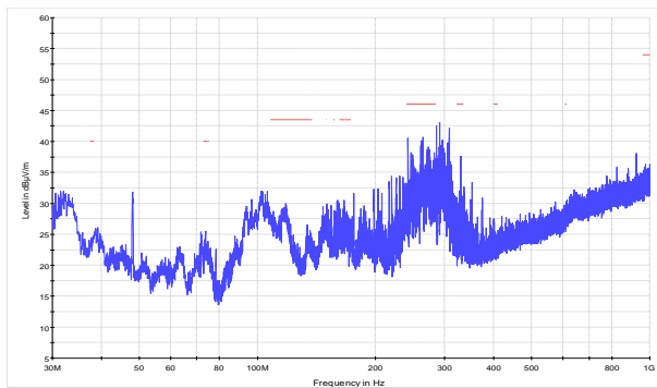
Figure 8.7-30: Radiated spurious emissions below 1 GHz for EDR2 modulation Mid channel
