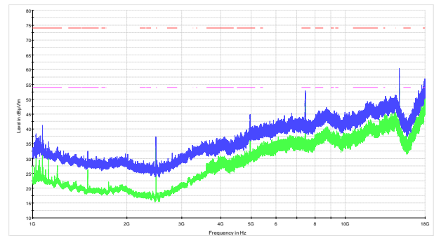
Figure 8.7-31: Radiated spurious emissions within 1–18 GHz for EDR2 modulation Mid channel
