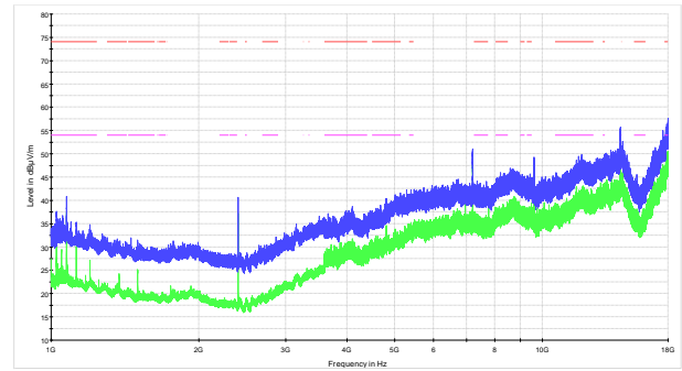
Figure 8.7-27: Radiated spurious emissions within 1–18 GHz for EDR2 modulation low channel
