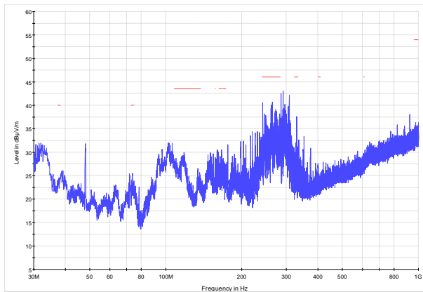
Figure 8.7-28: Radiated spurious emissions below 1 GHz for EDR2 modulation Mid channel
