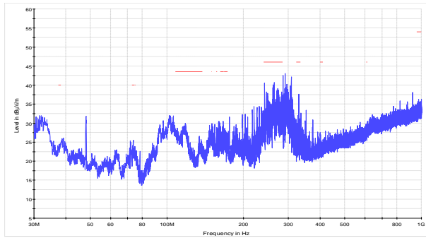
Figure 8.7-26: Radiated spurious emissions below 1 GHz for EDR2 modulation low channel
