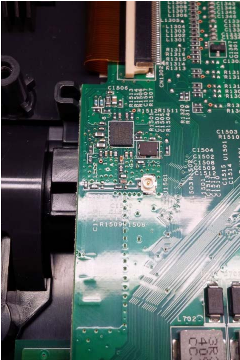
Figure 11: 9641GS Close-up of the Bluetooth radio section
