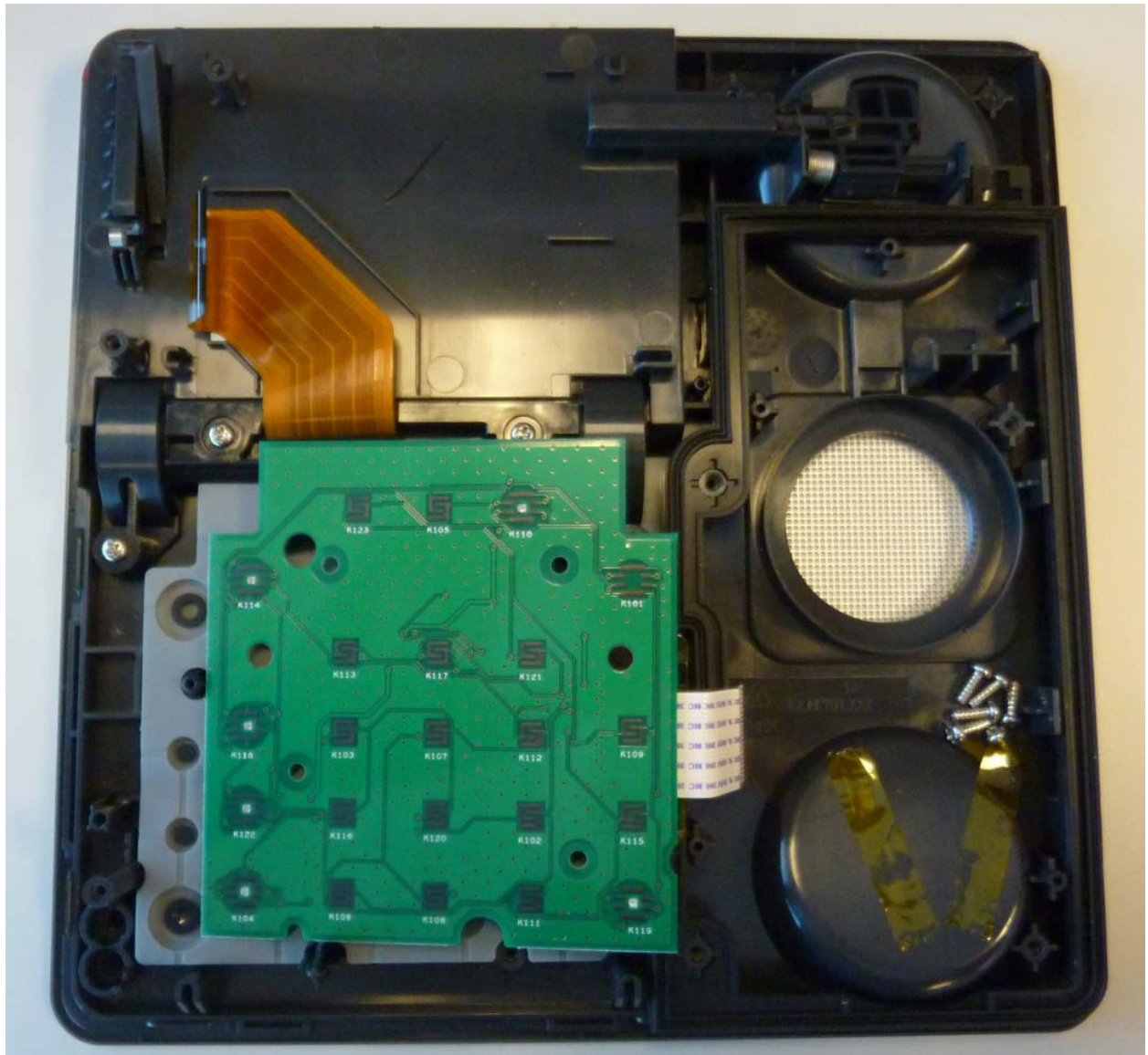
Figure 10: 9641GS Secondary side of keyboard
