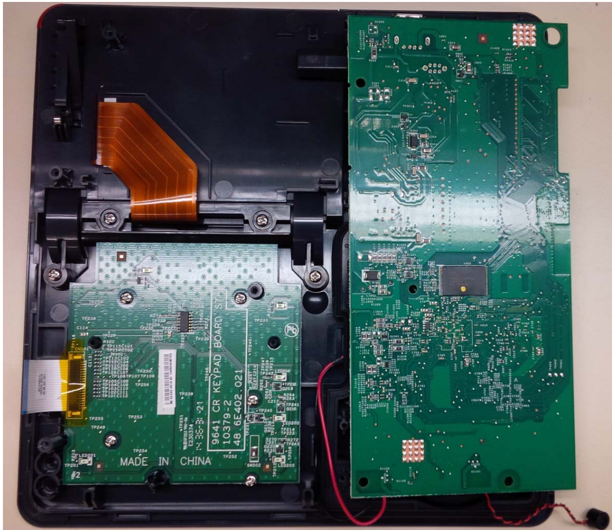
Figure 9: 9641GS Secondary side of motherboard (right).
