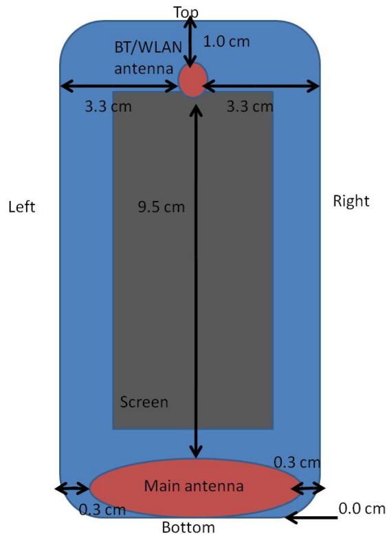
Figure 11-1 Identification of Sides for SAR Testing
