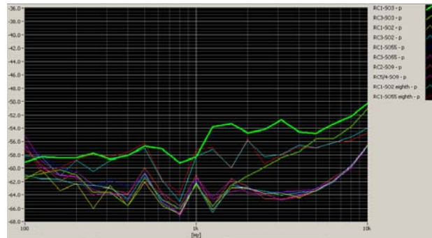
Figure 7-1 CDMA2000 Audio Band Magnetic Noise
