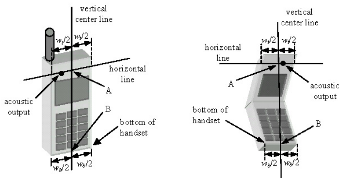
Figure 8-4 Handset Vertical Center & Horizontal Line Reference Points
