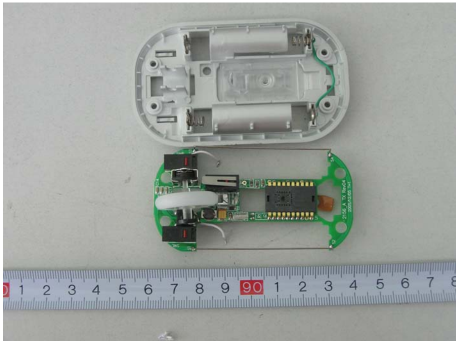
EUT-Inside View (2)
