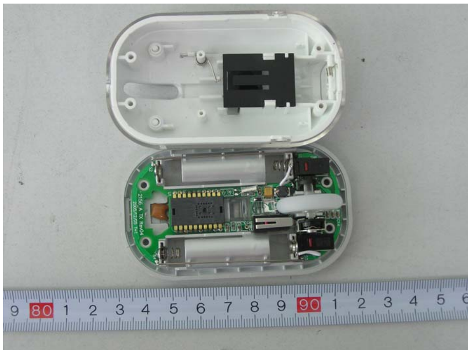
EUT-Inside View (1)
