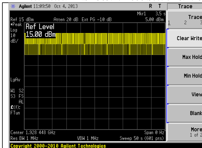
EUT transmits on interference free time-slot
