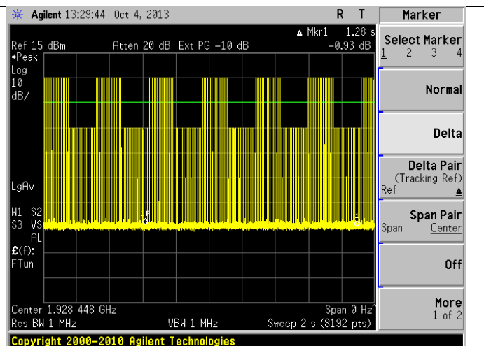
EUT pauses every 1.28 seconds
