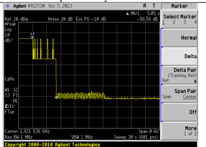
EUT ceases transmissions within 5 sec
