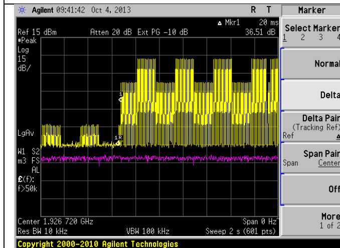
Change of channel with interference introduced
