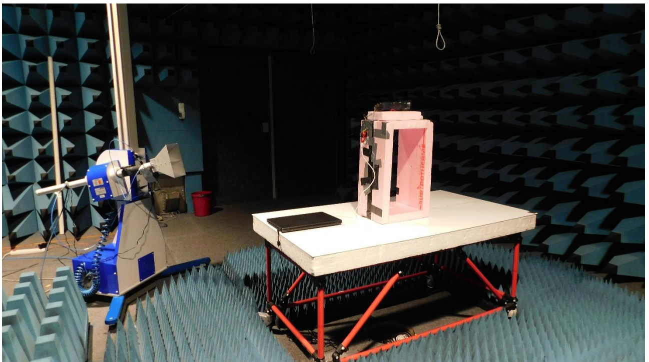
Picture 6: AC, radiated emission test 1 GHz – 17 GHz (rear view)
