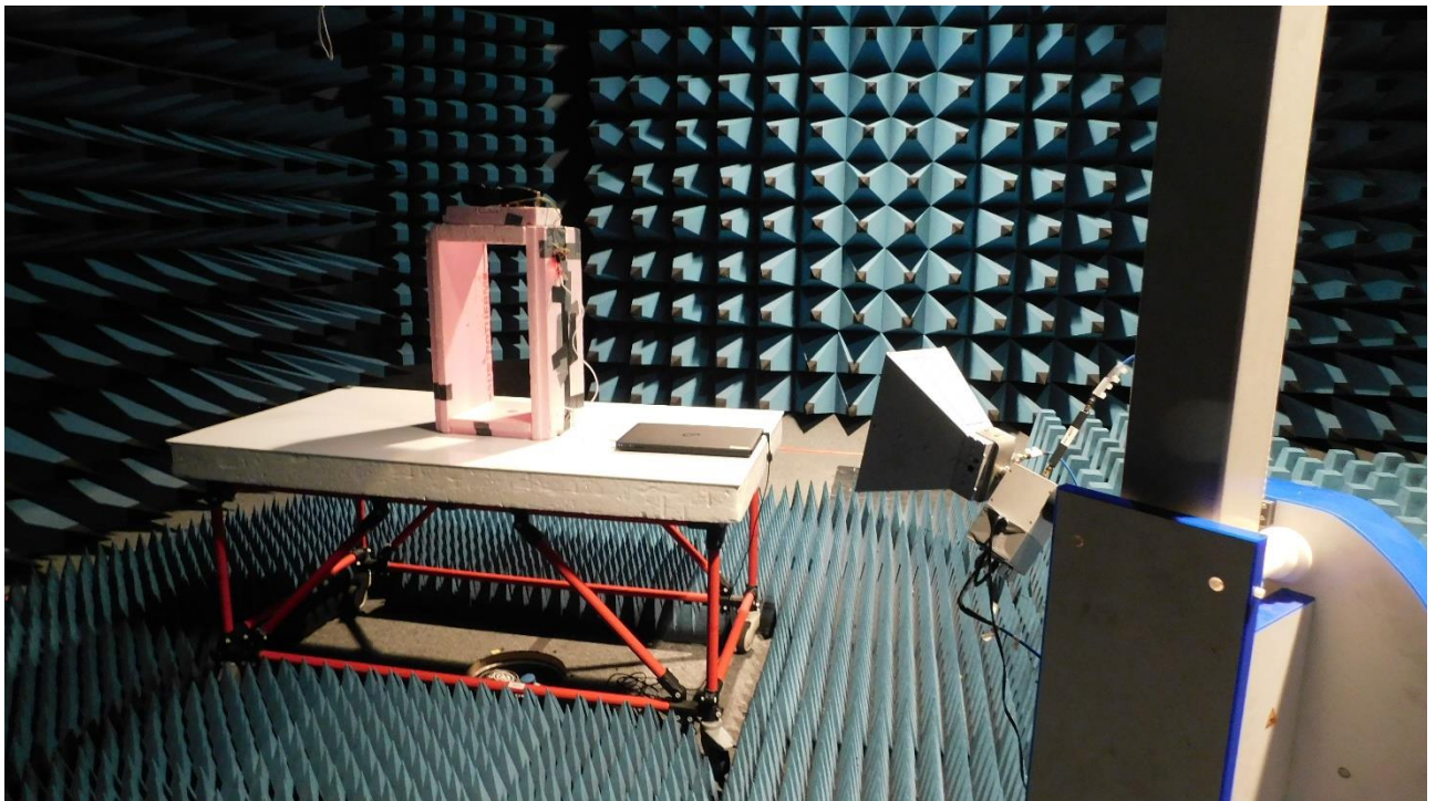
Picture 5: AC, radiated emission test 1 GHz – 17 GHz (front view)
