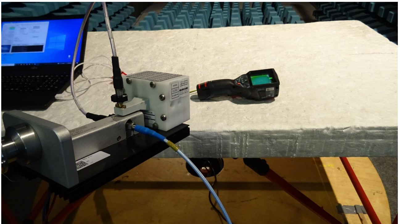
Picture 7: AC, exploratory measurement 17 GHz – 25 GHz (front view)
