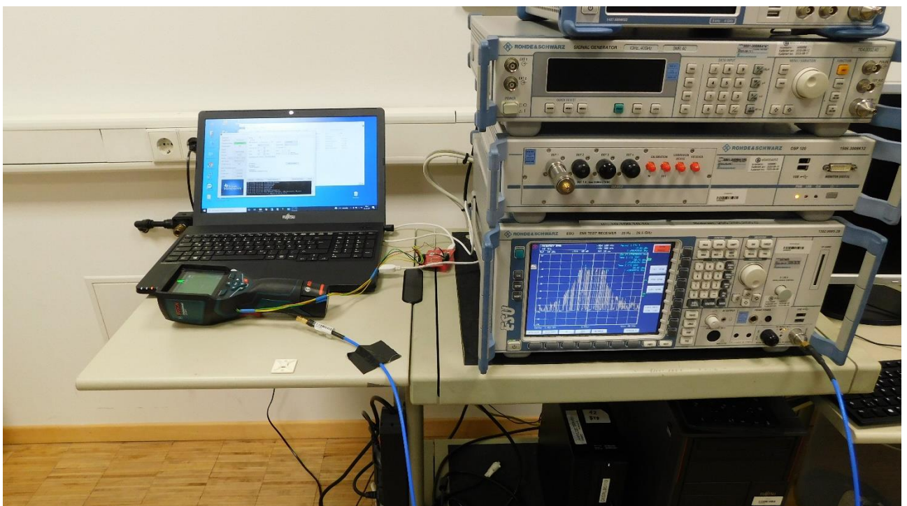
Picture 8: Conducted measurements (occupied bandwidth, band edge and antenna-port measurements)
