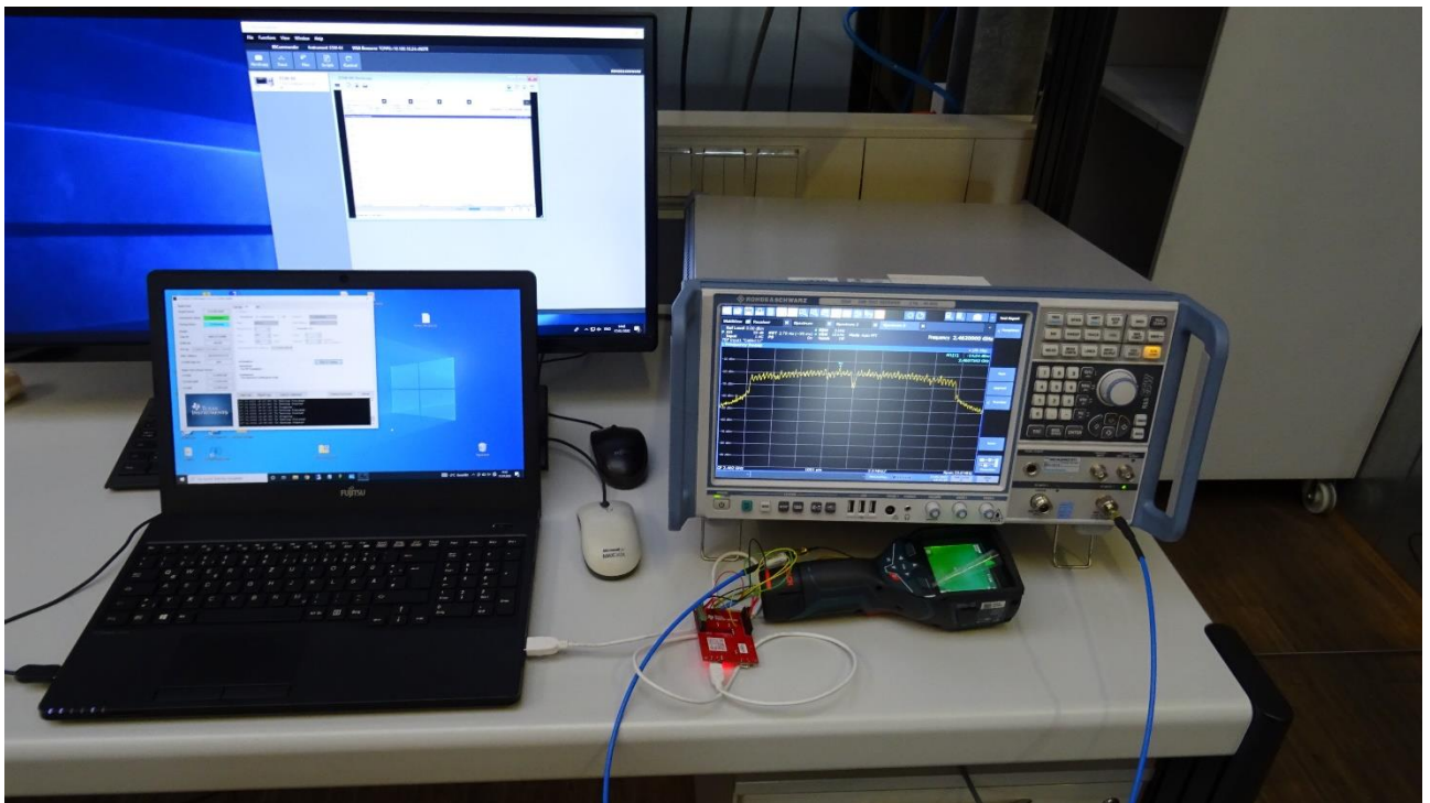
Picture 9: Conducted measurements (6 dB bandwidth, conducted output power and power spectral density measurements)
