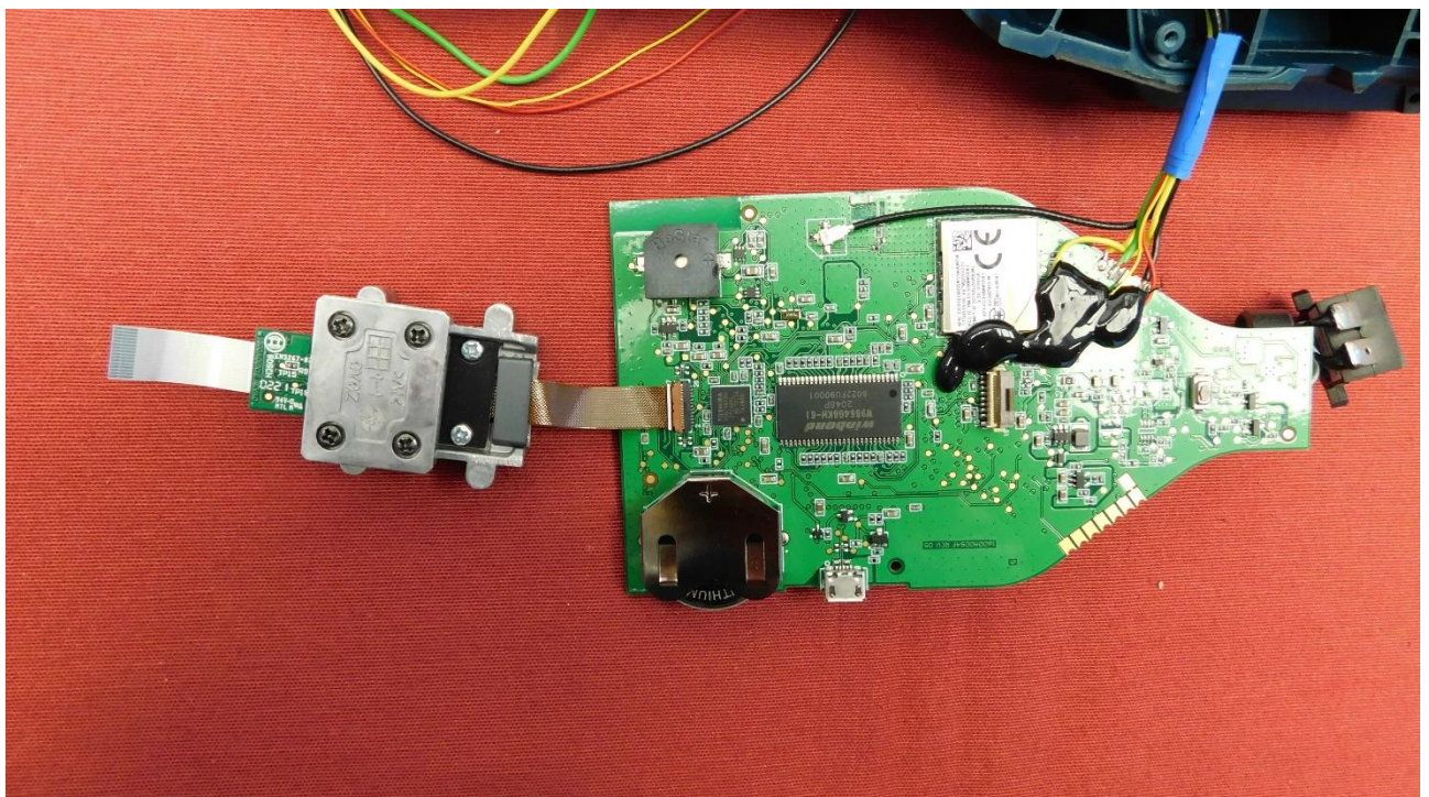
Picture 6: Rear view of module
