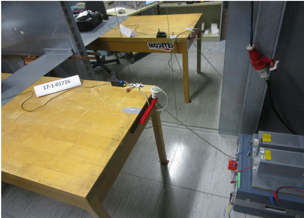
Photograph 1: EMI-AC measurements
