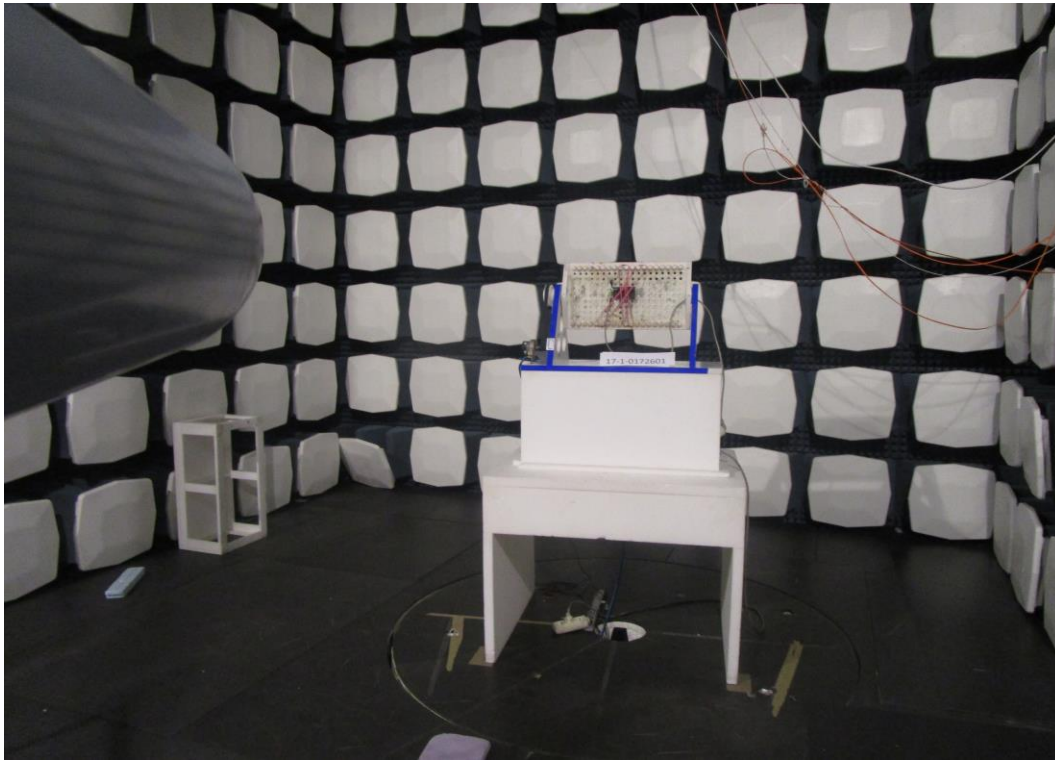
Photograph 3: EUT Measurements in the anechoic chamber, Radiated interference field strength test set-up 2
