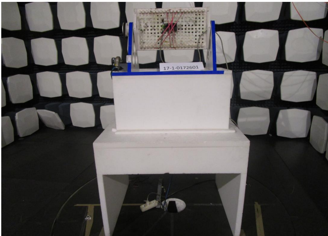
Photograph 2: EUT Measurements in the anechoic chamber, Radiated interference field strength test set-up 1
