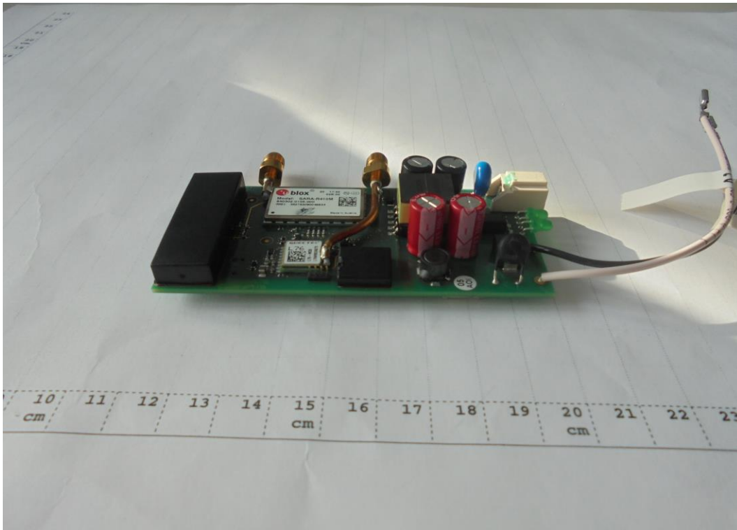
Photograph 5: EUT Inside Side View
