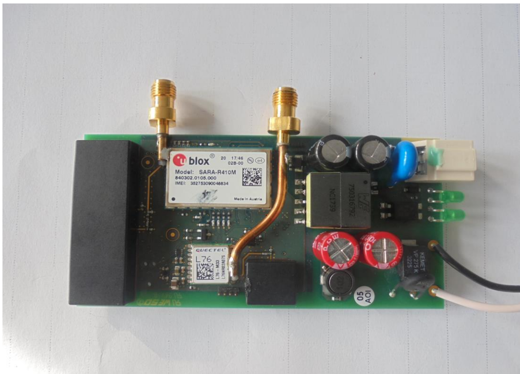
Photograph 2: EUT Inside Top View_2
