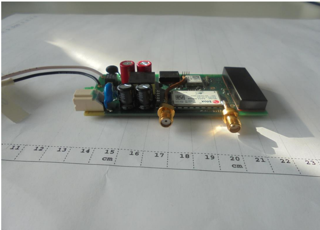
Photograph 4: EUT Inside Side View
