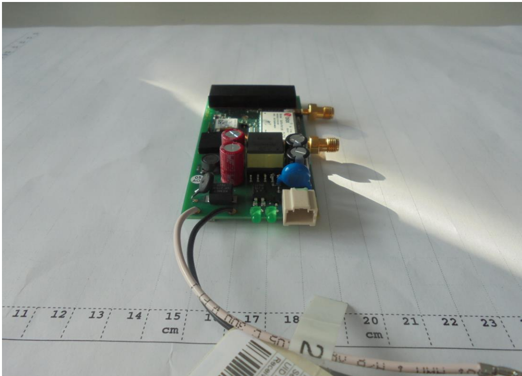
Photograph 7: EUT Inside Side View
