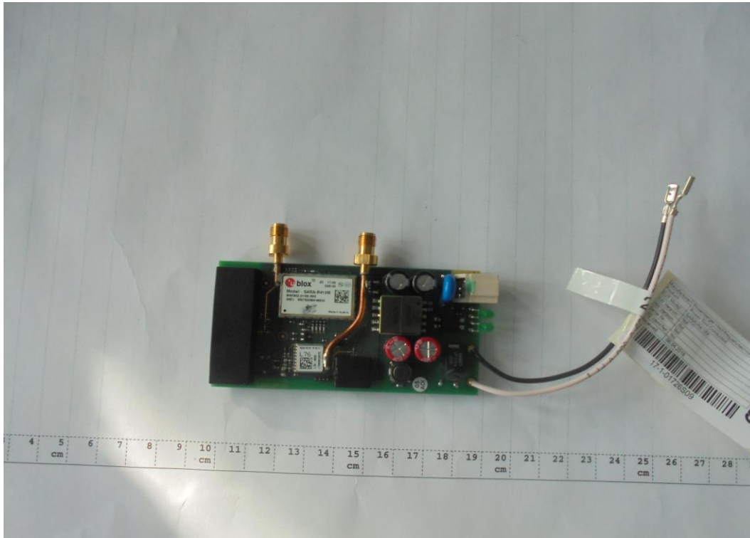
Photograph 1: EUT Inside Top View_1
