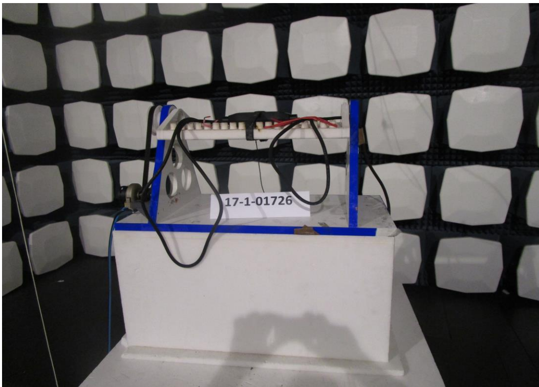
Photograph 2: EUT Measurements in the anechoic chamber, Radiated interference field strength test set-up
