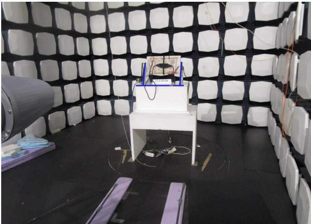
Photograph 4: EUT Measurements in the anechoic chamber, Radiated interference field strength test set-up
