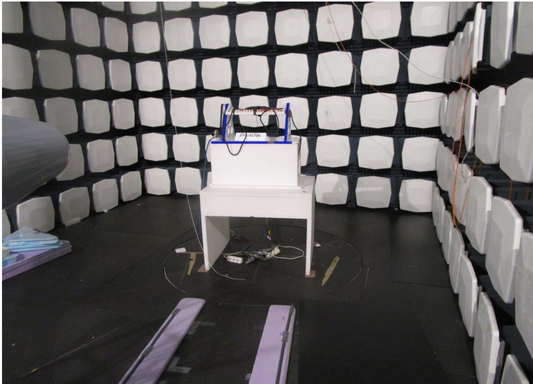
Photograph 3: EUT Measurements in the anechoic chamber, Radiated interference field strength test set-up
