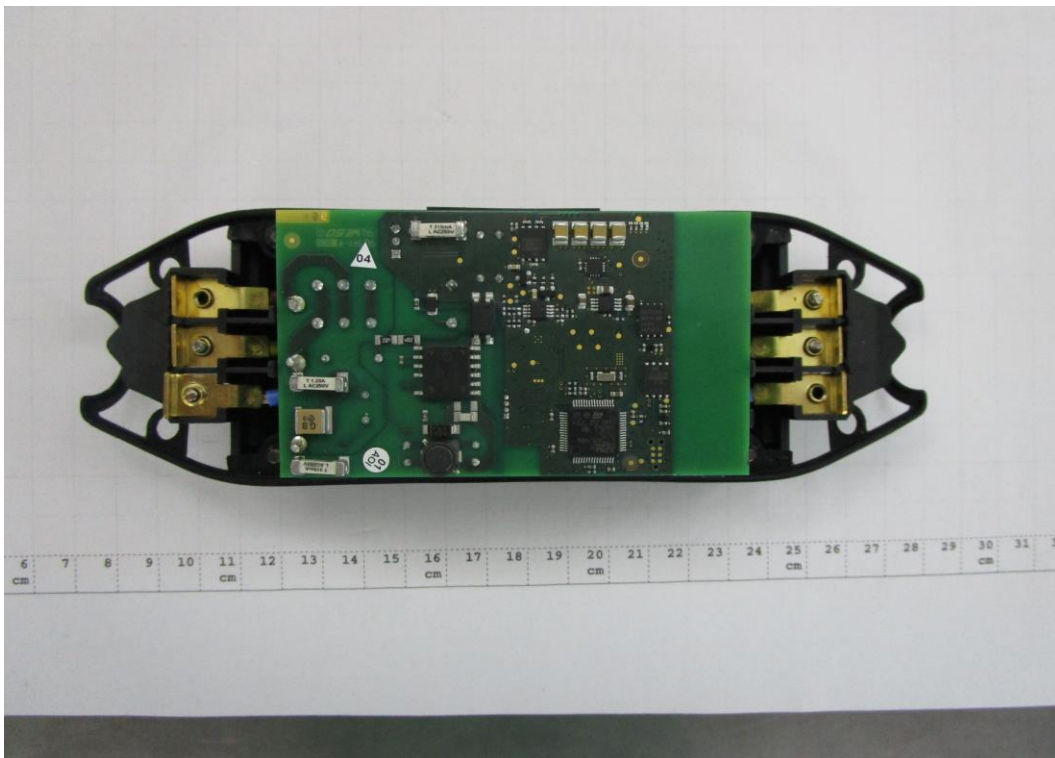
Photograph 2: EUT Inside
