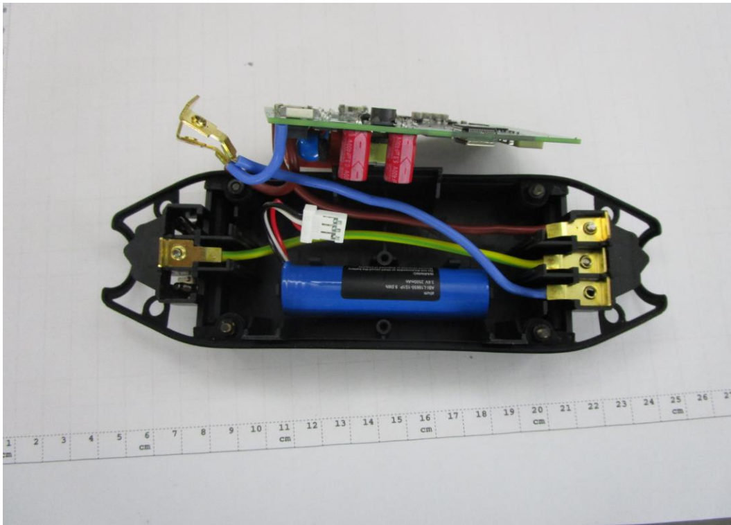
Photograph 3: EUT Inside
