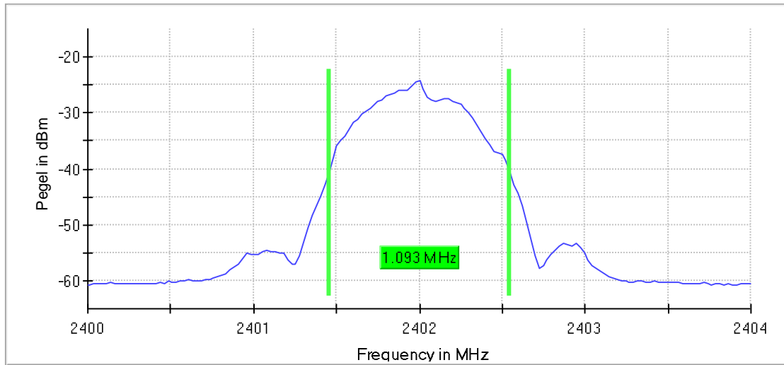
99%-BW, 2402 MHz
