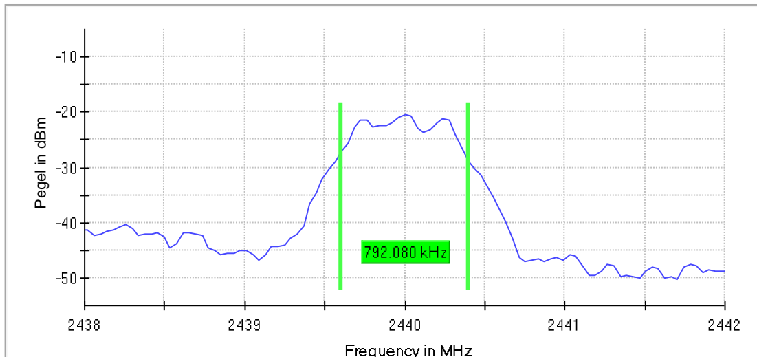
6dB-BW, 2440 MHz
