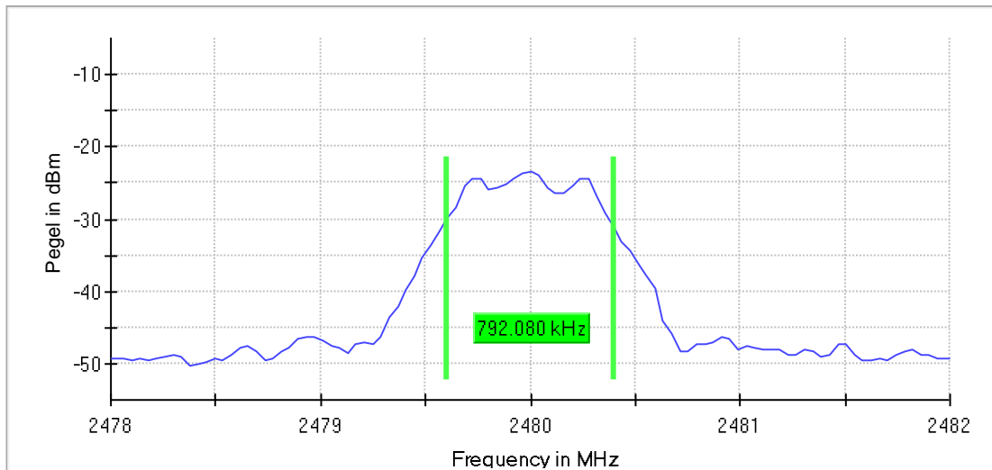
6dB-BW, 2480 MHz
