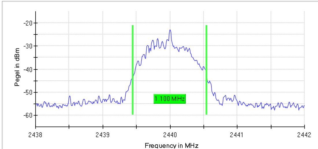
20dB-BW, 2440 MHz
