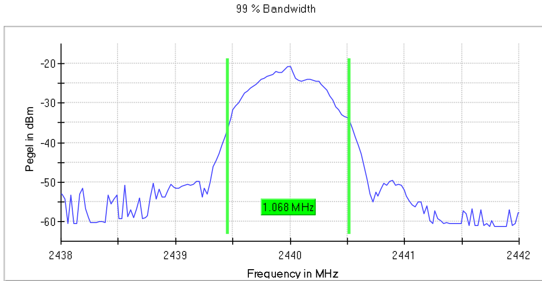
99%-BW, 2440 MHz
