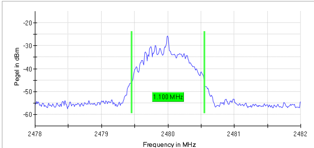
20dB-BW, 2480 MHz
