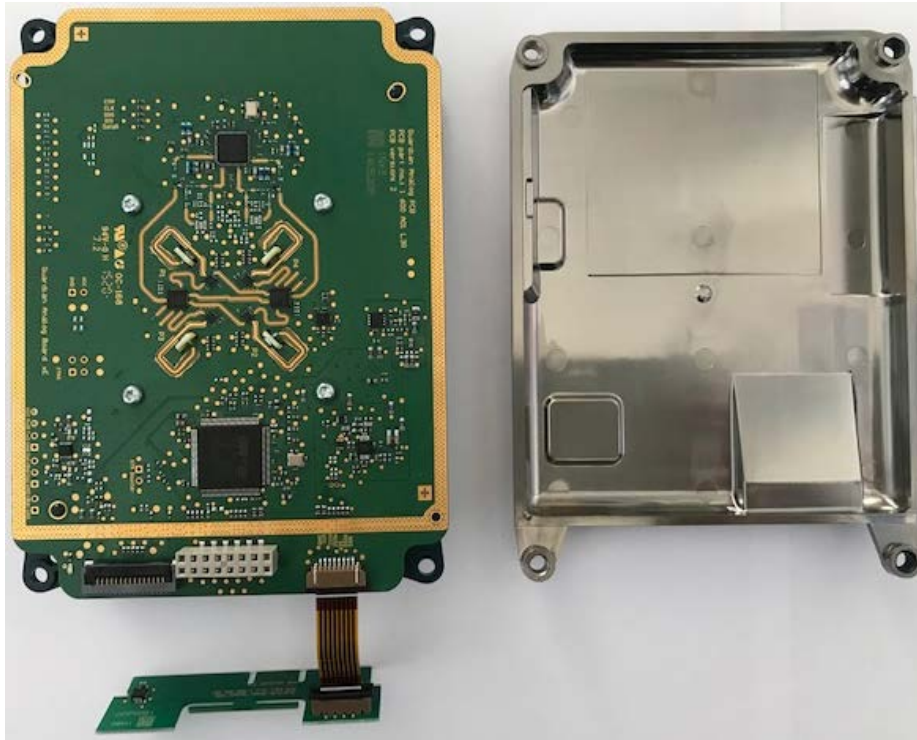
Sensor frontend (left), Shield (right)
