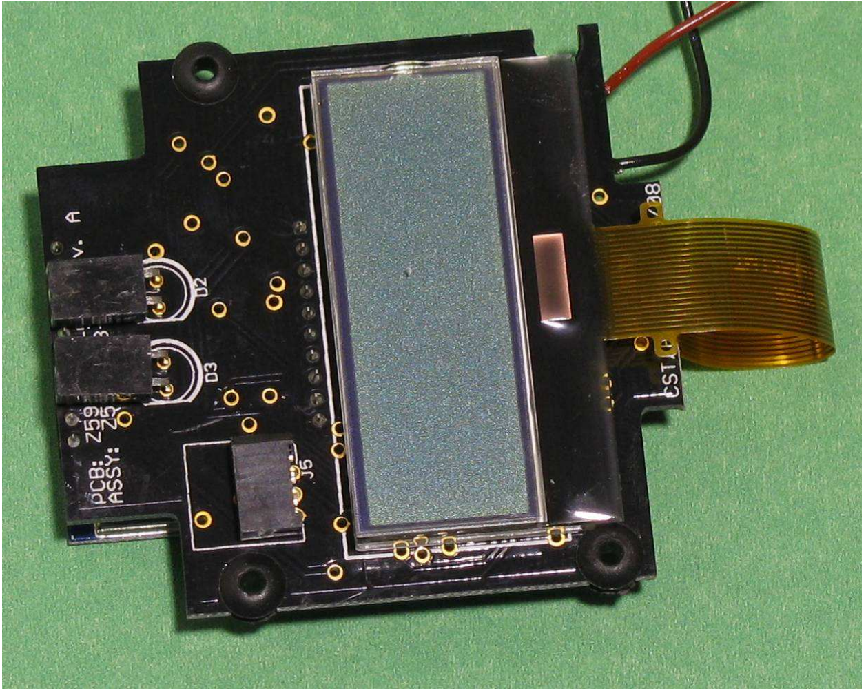
Front Side of Circuit Board Showing LCD
