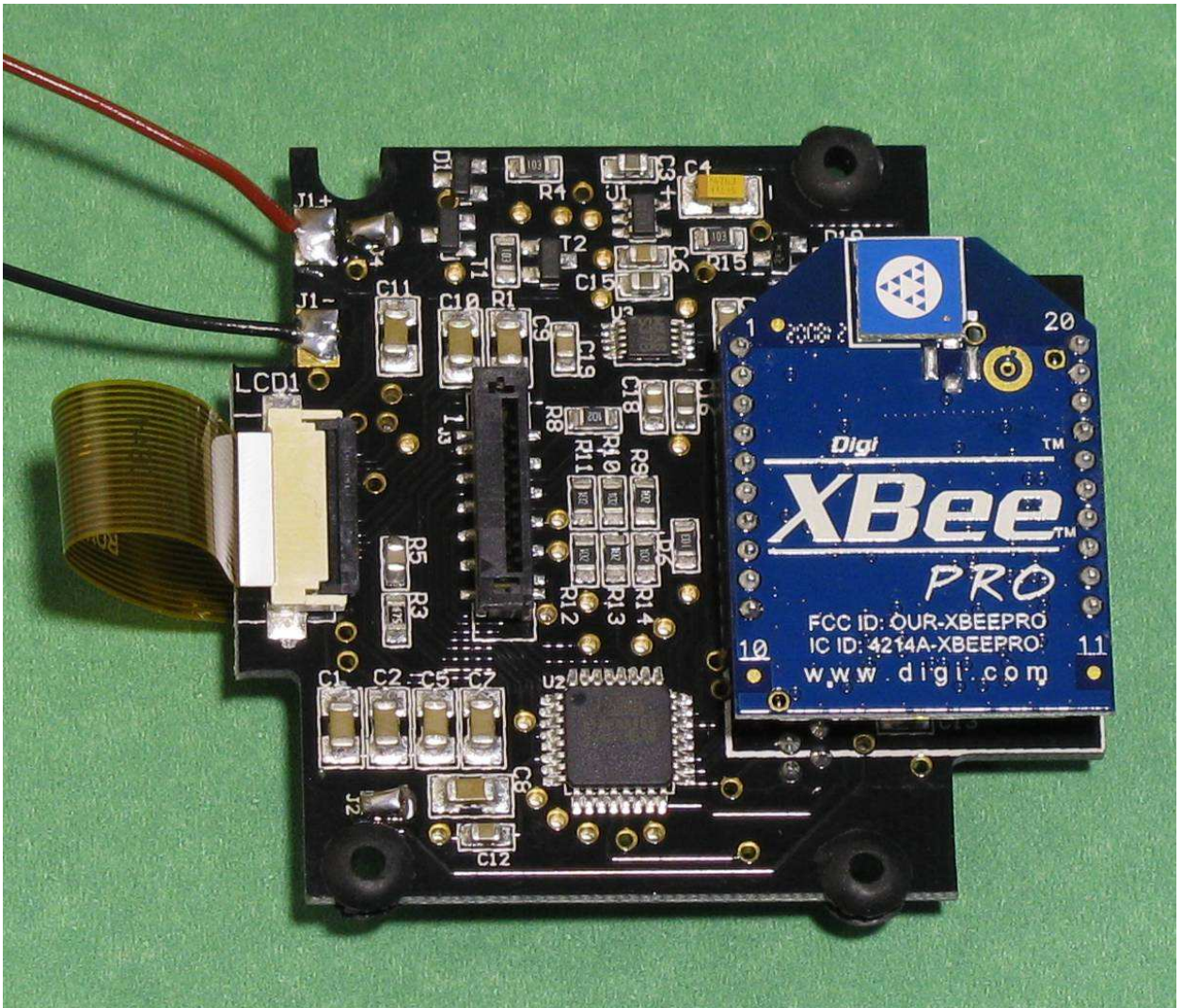
Circuit Boards Showing Transmitter Module
