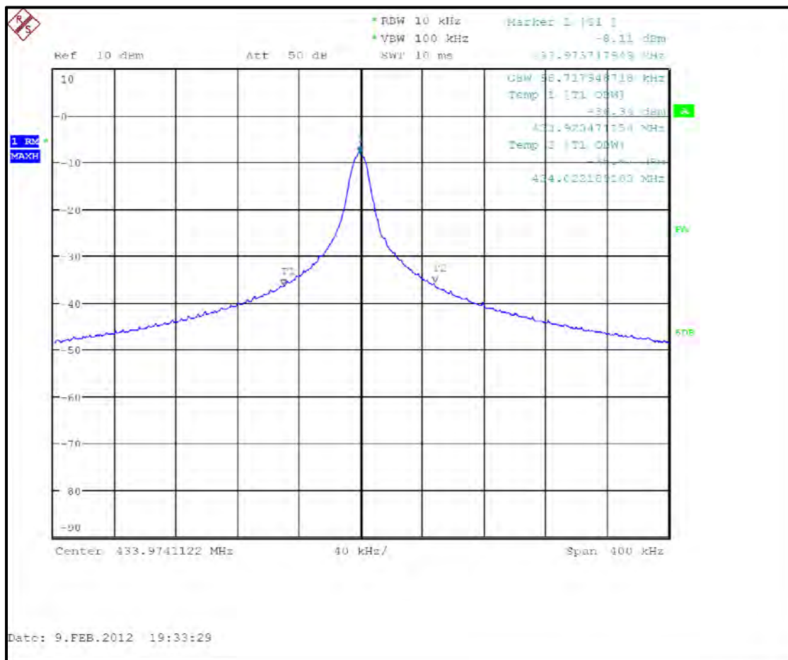
Plot 5-2: Modulated Bandwidth – 99%
