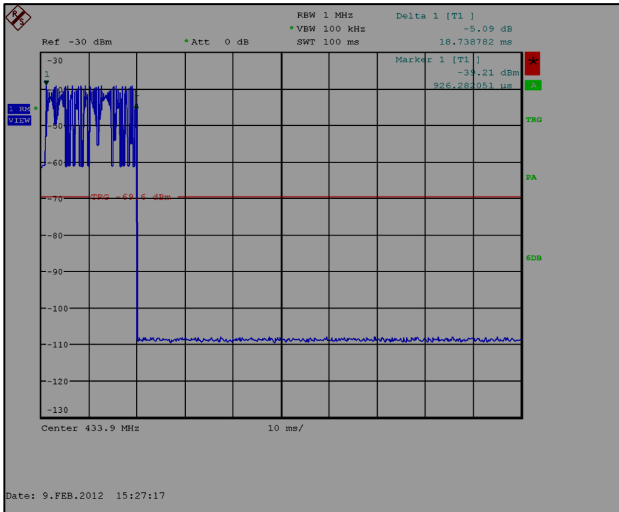
Plot 3-1: Transmit on in 100 ms Window
