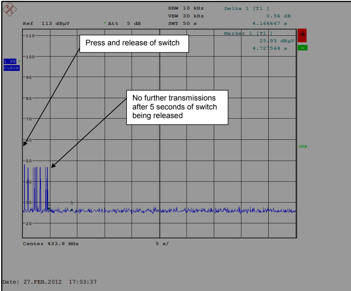
Plot 4-1: Transmitter Deactivation
