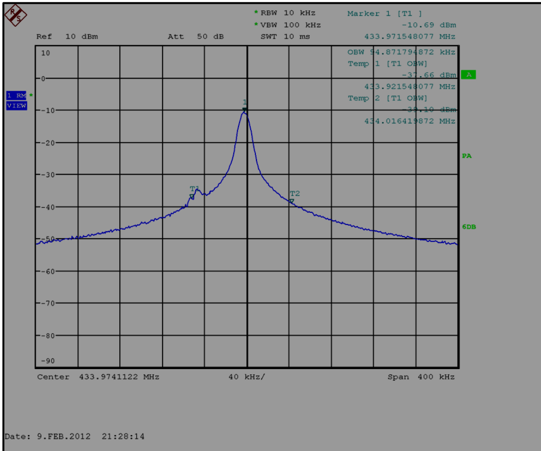
Plot 5-2: Modulated Bandwidth – 99%
