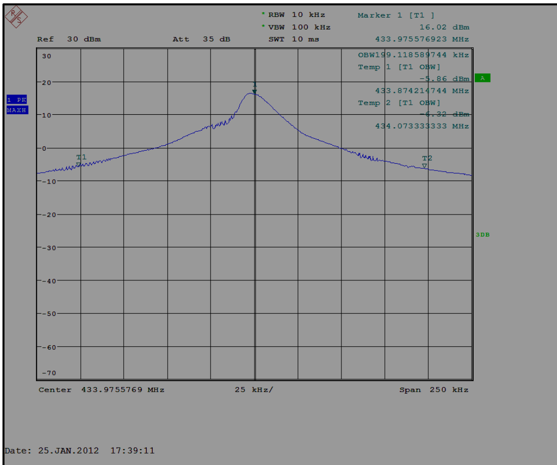
Plot 5-1: Modulated Bandwidth – 20 dB
