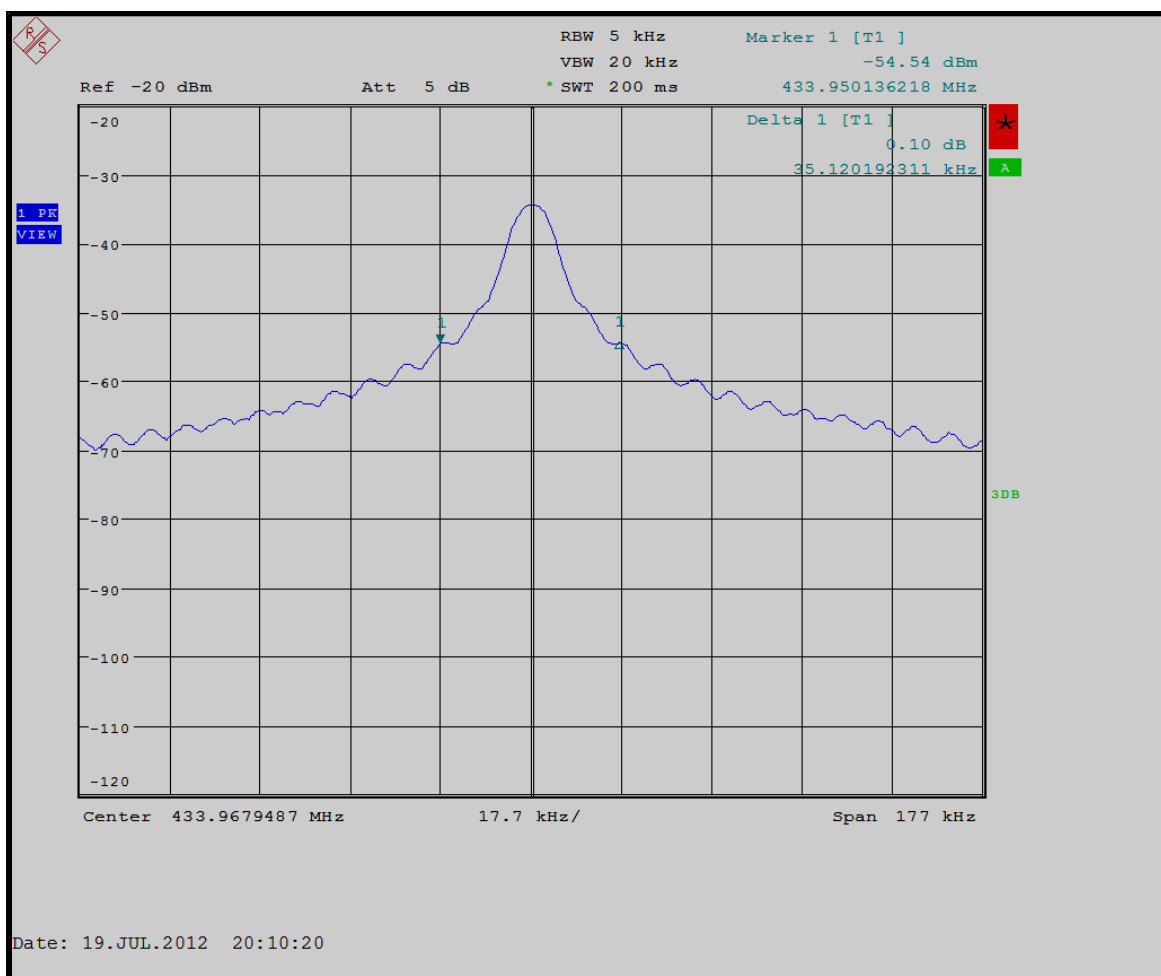
Plot 5-1: Modulated Bandwidth
