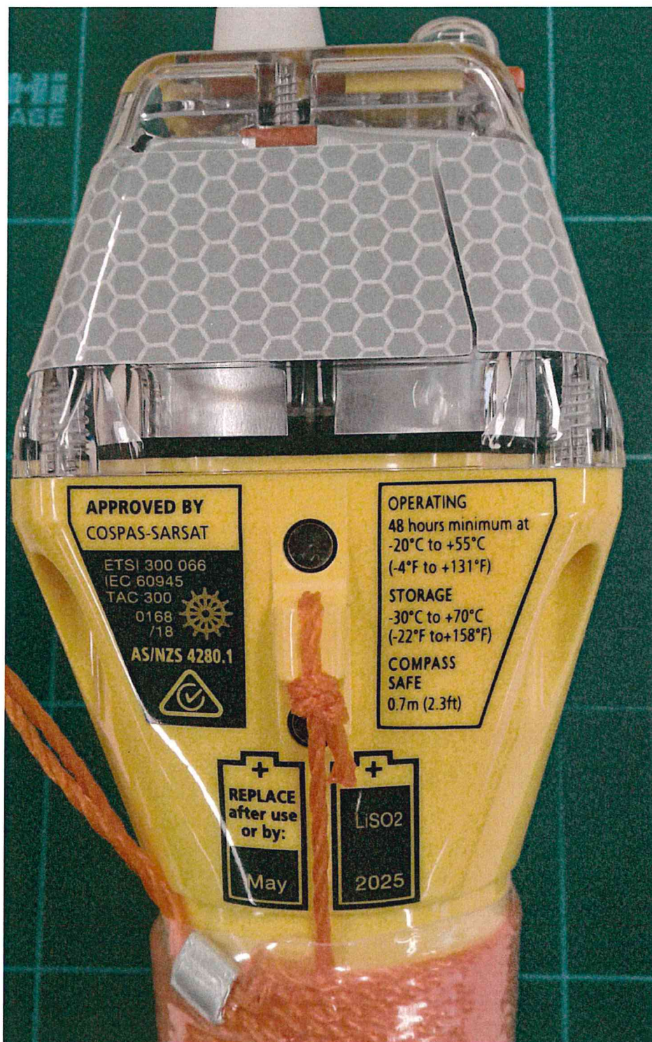
Figure 6 EPIRB face E - after laser etching
