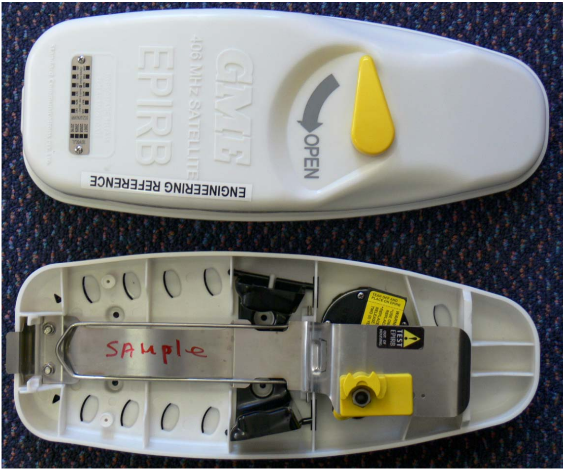
Picture 7 - Auto-release Housing, Cover and Base (MT403FF/403FG)
