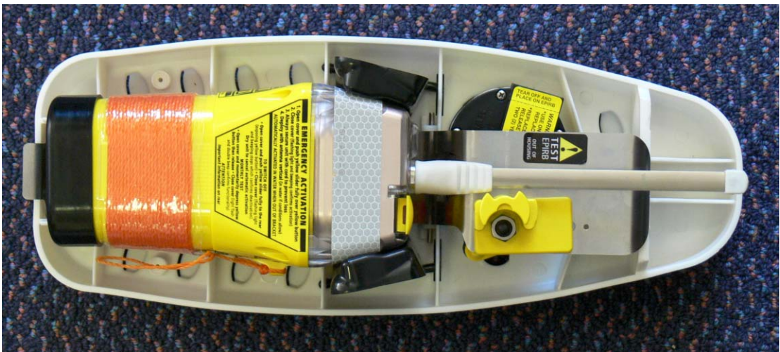
Picture 8 - EPIRB in Auto-release housing, cover removed (MT403FF/403FG)
