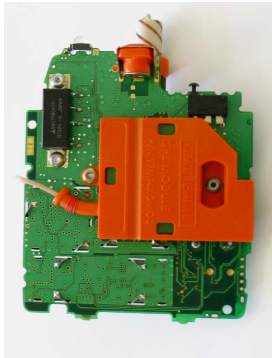
MT403 CCA with GPS module fitted
