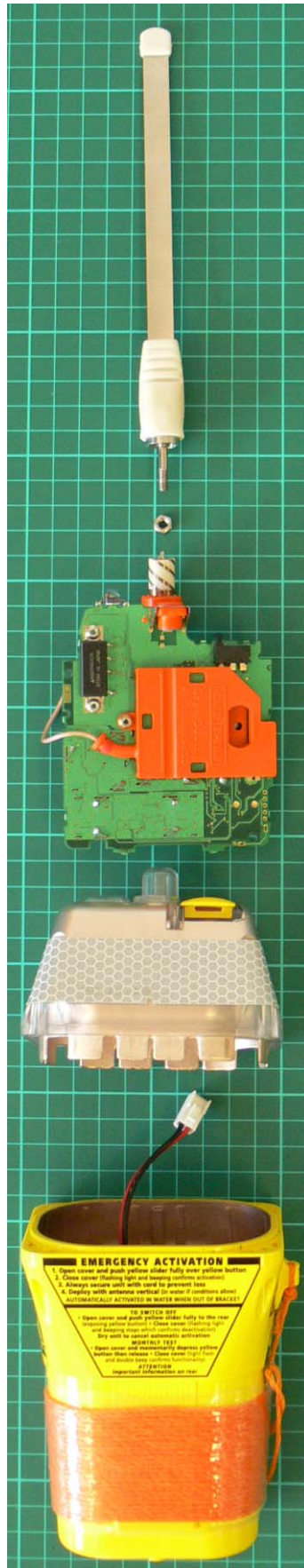
Picture 4 - Exploded view (MT403G shown)
