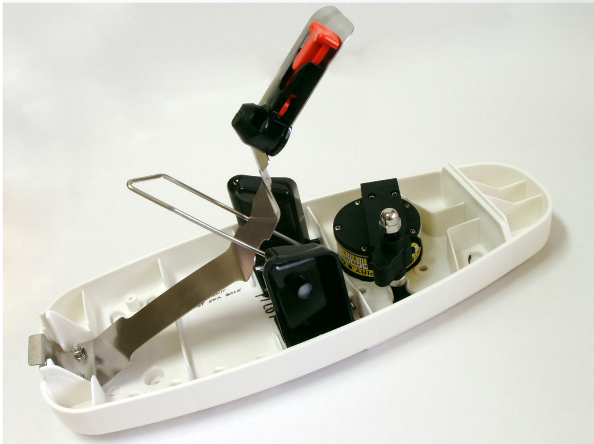
Figure 11 - MT401FF Auto-release housing, misc views
