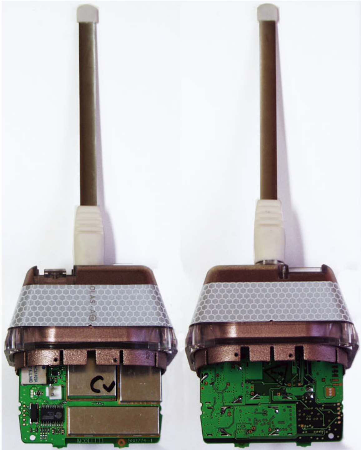
Figure 2 - Cap assembly view (front & rear)
