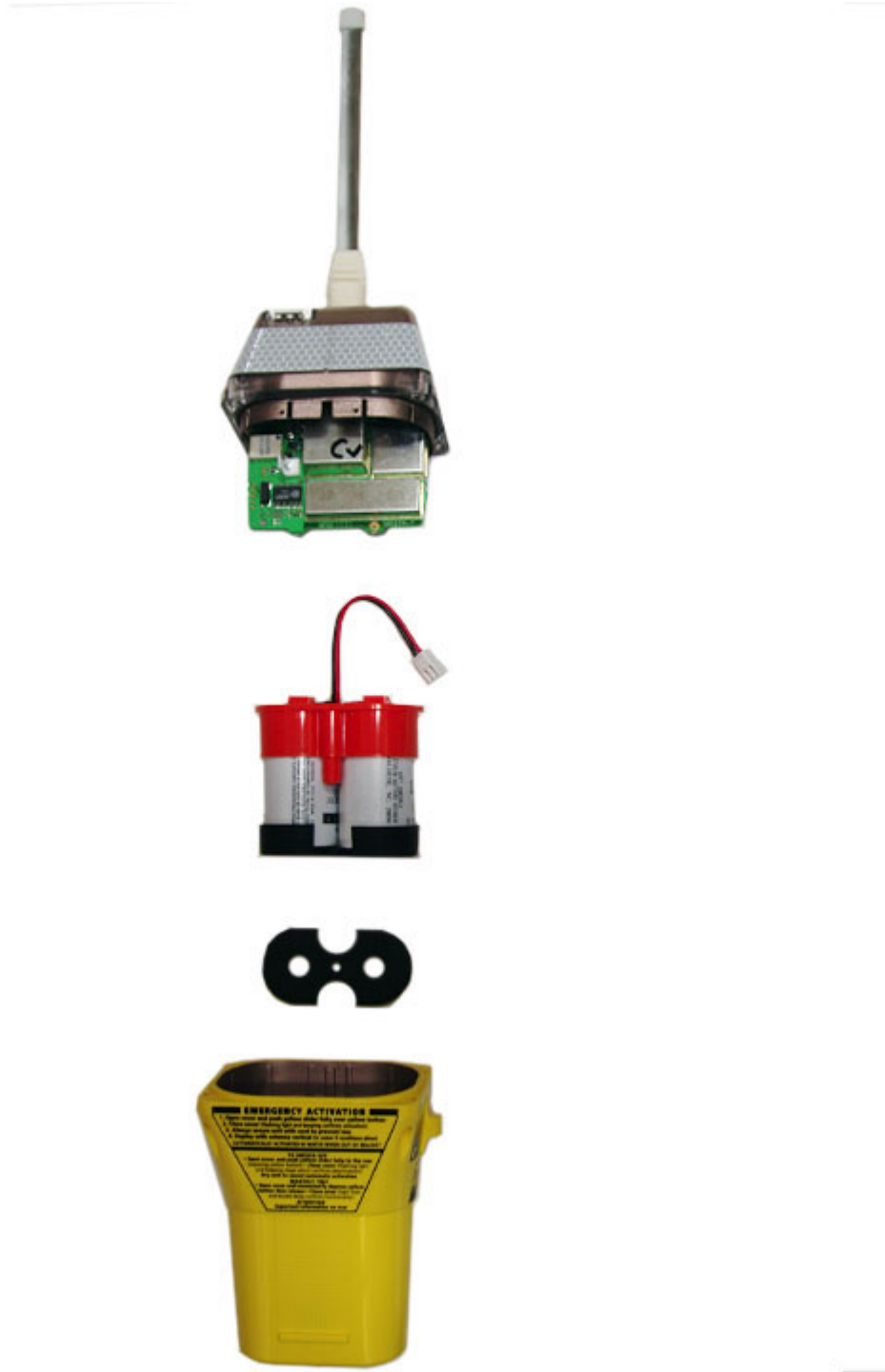
Figure 1 - Exploded assembly view
