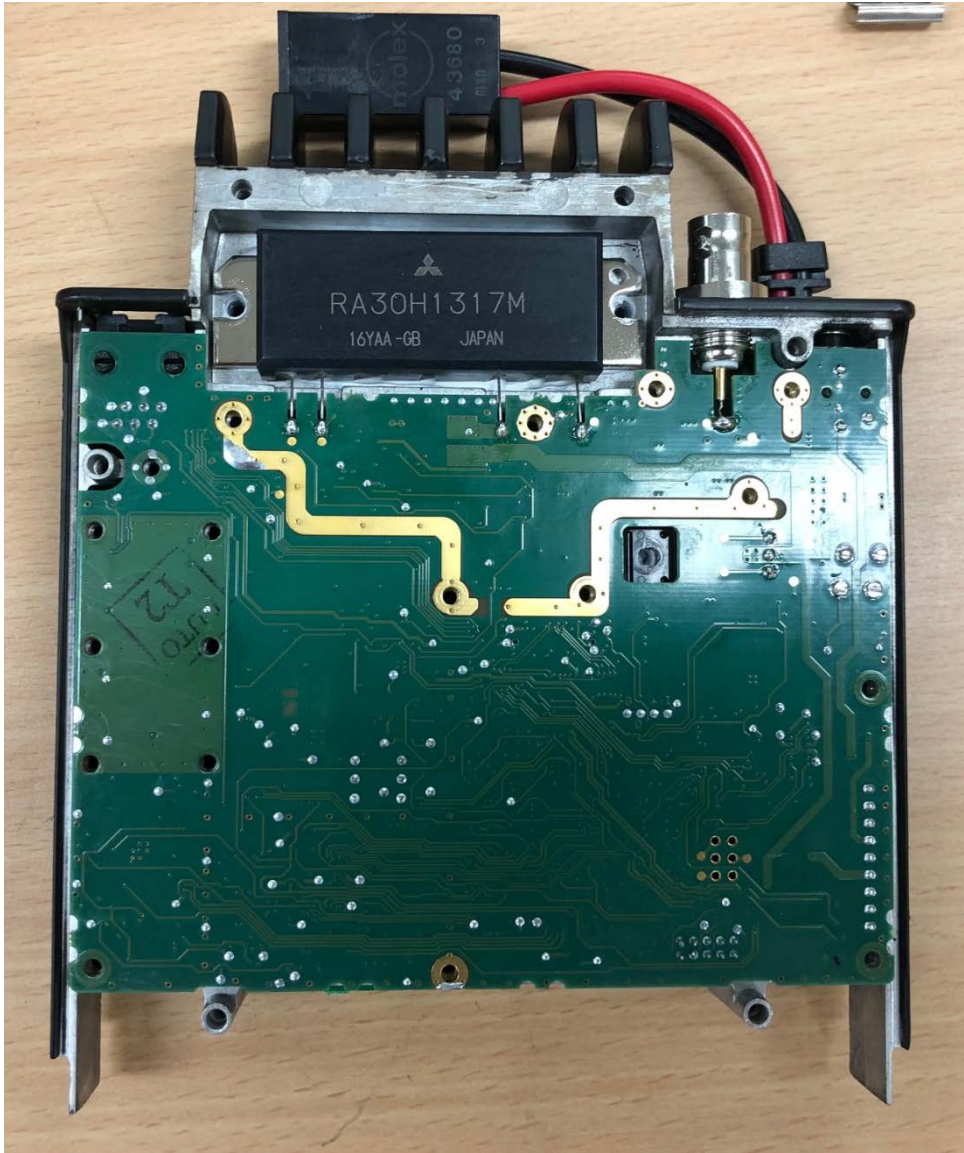
Bottom Main Board
