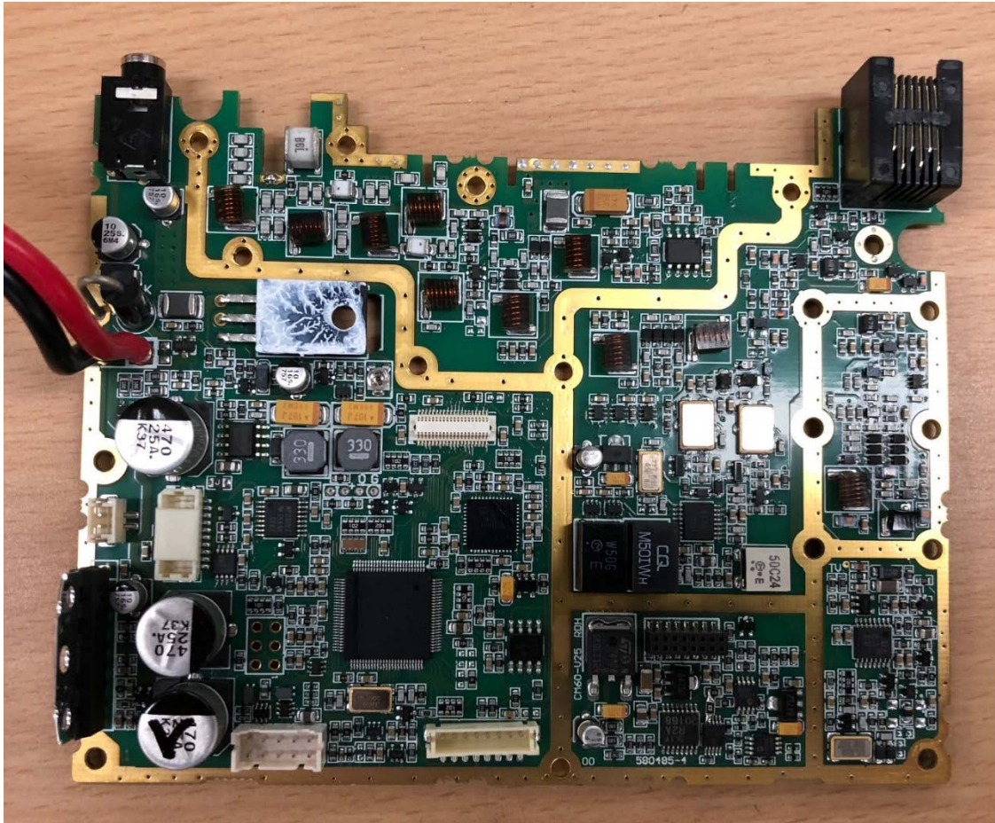
Top main Board
