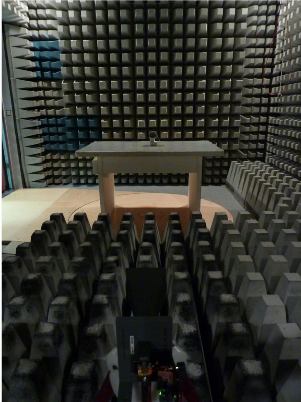
123441_7.JPG: Test setup fully anechoic chamber
