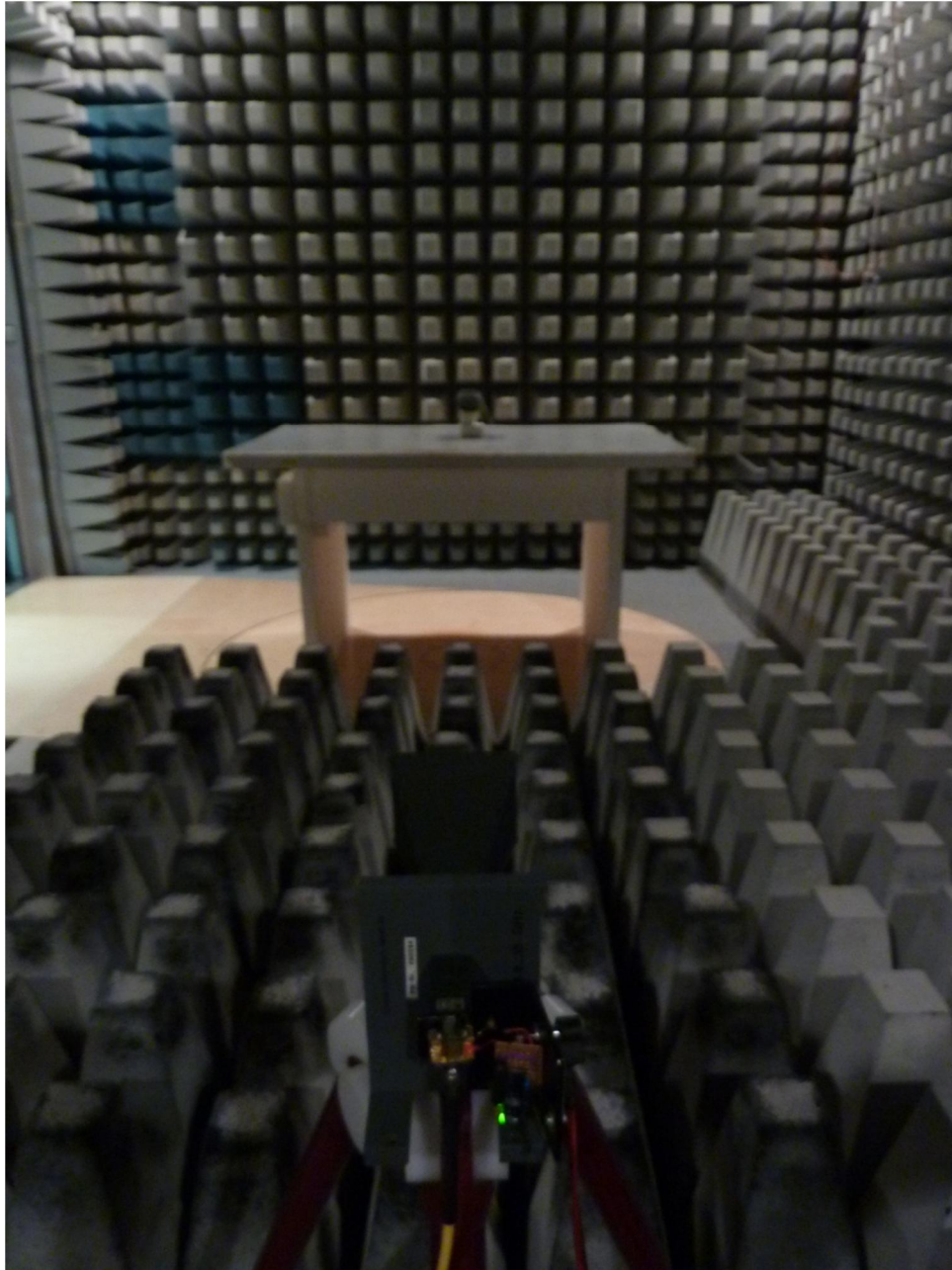
123441_6.JPG: Test setup fully anechoic chamber
