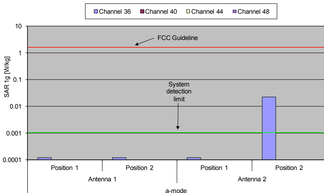
Fig. 9: The measured body SAR values for the Cognex MD9500 for IEEE 802.11 a in body worn configuration, in comparison to the FCC exposure limit.
