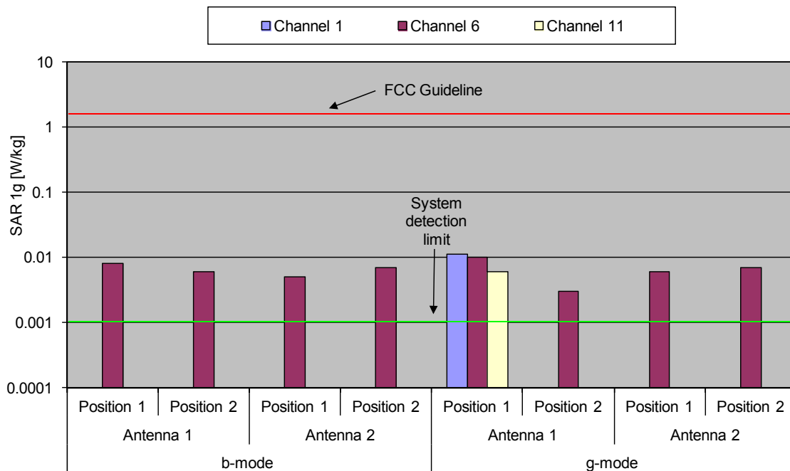
Fig. 8: The measured body SAR values for the Cognex MD9500 for IEEE 802.11 b/g in body worn configuration, in comparison to the FCC exposure limit.
