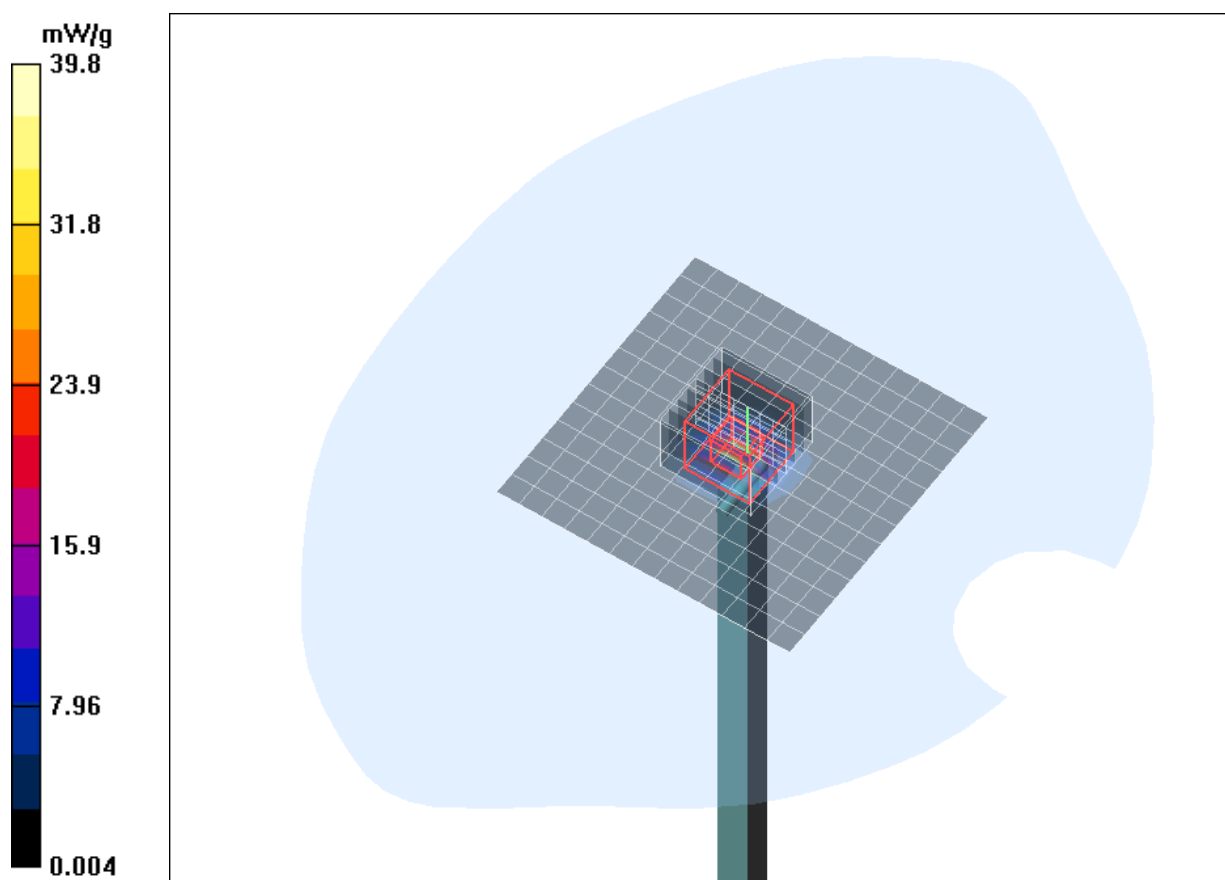
Fig. 11: Validation measurement 5200 MHz Body (June 25, 2012) coarse grid. Ambient Temperature: 21.9°C. Liquid Temperature: 21.8°C.
