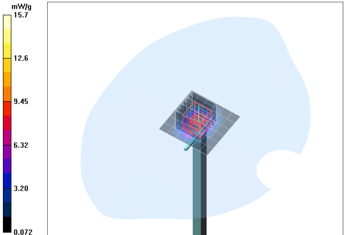
Fig. 10: Validation measurement 2450 MHz Body (June 19, 2012) coarse grid. Ambient Temperature: 22.4°C. Liquid Temperature: 22.2°C.
