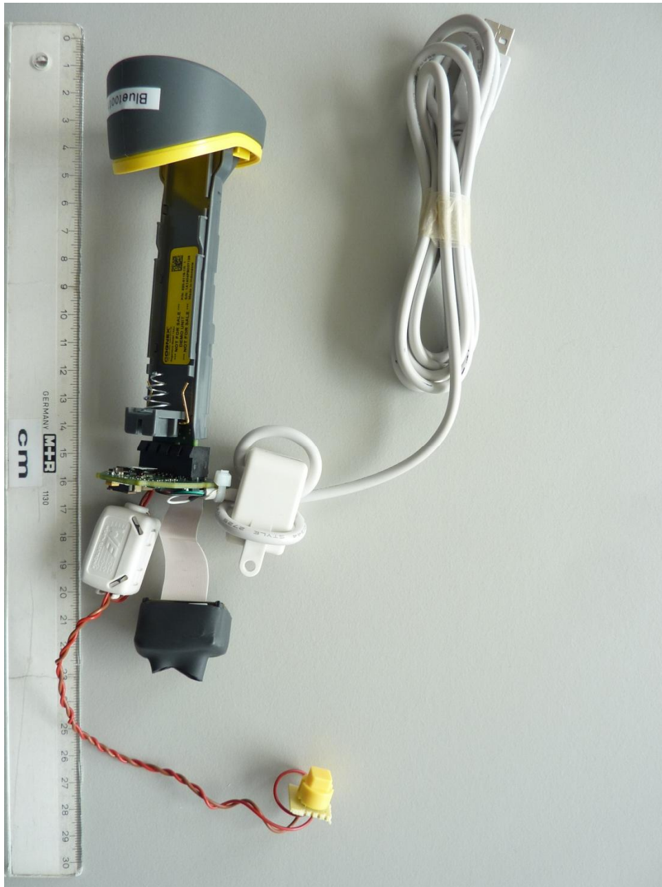
140269_8.JPG: Bluetooth Slide-in connected with ancillary programming PCB
