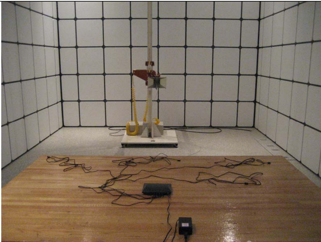
Radiated Emissions(1000MHz~1800MHz)
