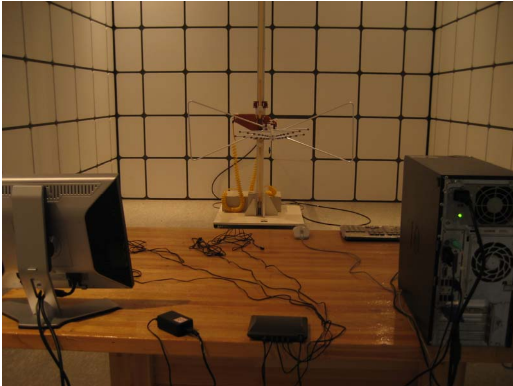
Radiated Emissions(30MHz~1000MHz) - Serial Communication Mode
