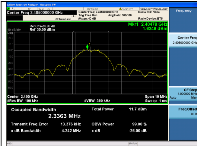
99% Bandwidth - Mid CH 2405
